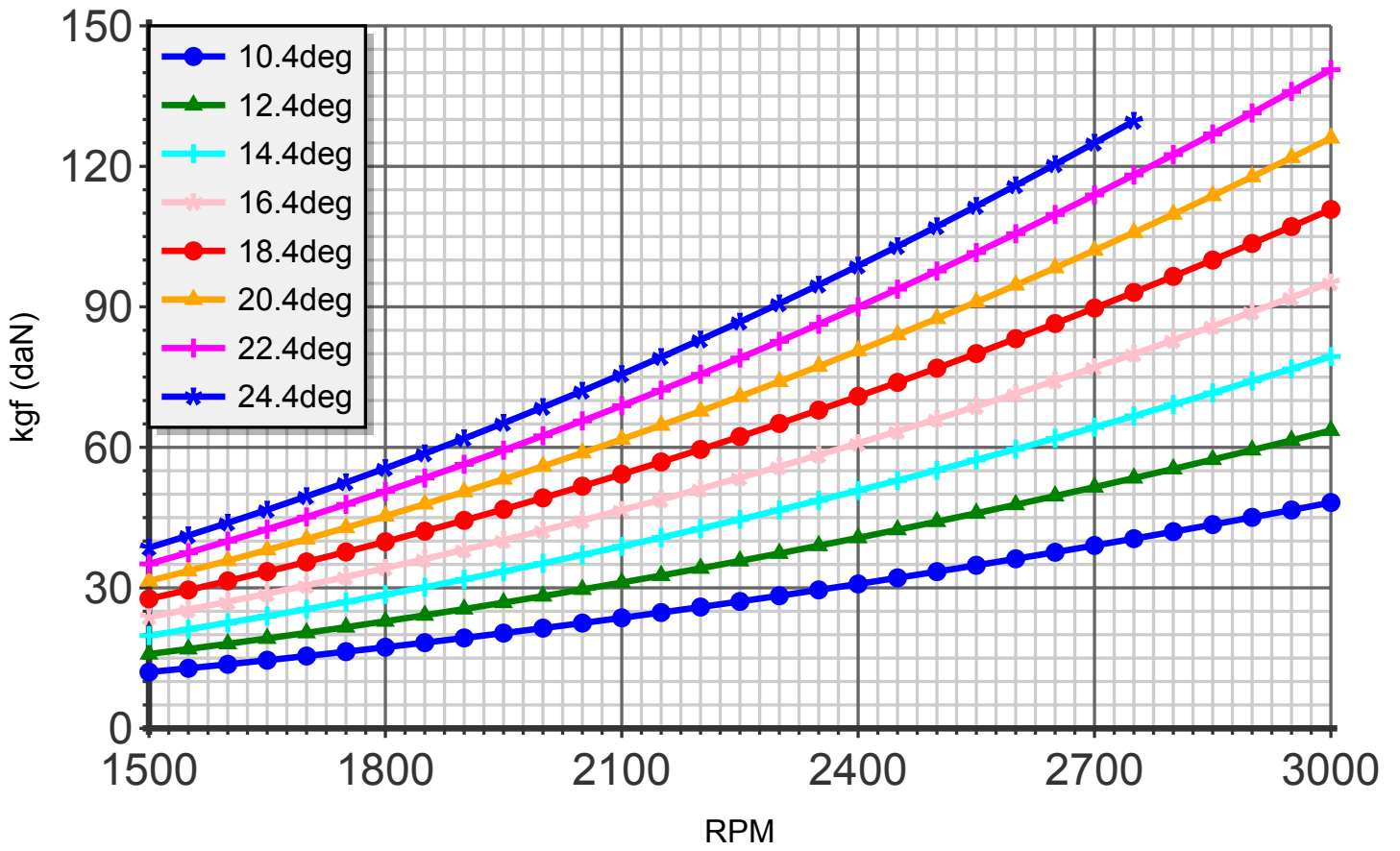
Thrust (blade:2 diameter:150cm R-1300)
