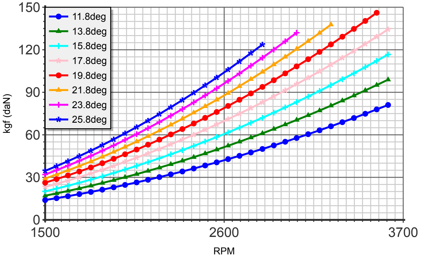
Thrust (blade:2 diameter:135cm R-1100)
