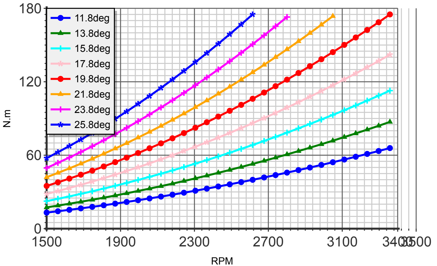
Torque (blade:3 diameter:145cm R-1100)
