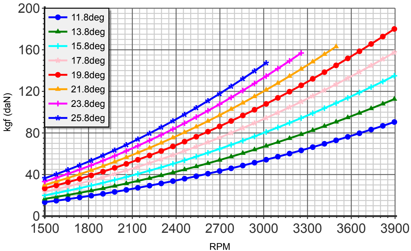
Thrust (blade:3 diameter:125cm R-0600)
