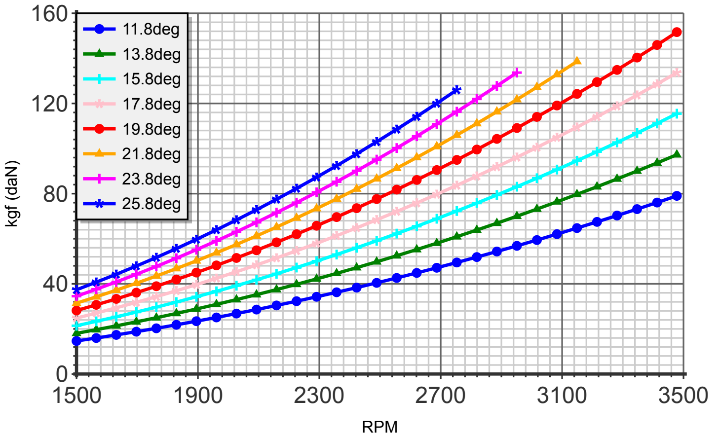
Thrust (blade:2 diameter:140cm R-1100)
