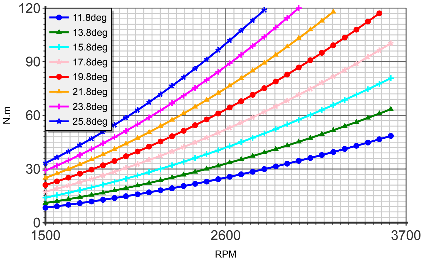
Torque (blade:2 diameter:135cm R-1100)
