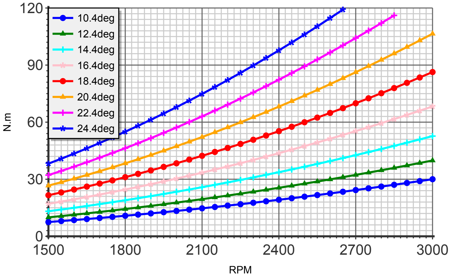
Torque (blade:2 diameter:160cm R-1300)
