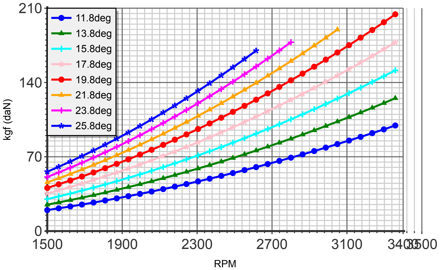
Thrust (blade:3 diameter:145cm R-1100)
