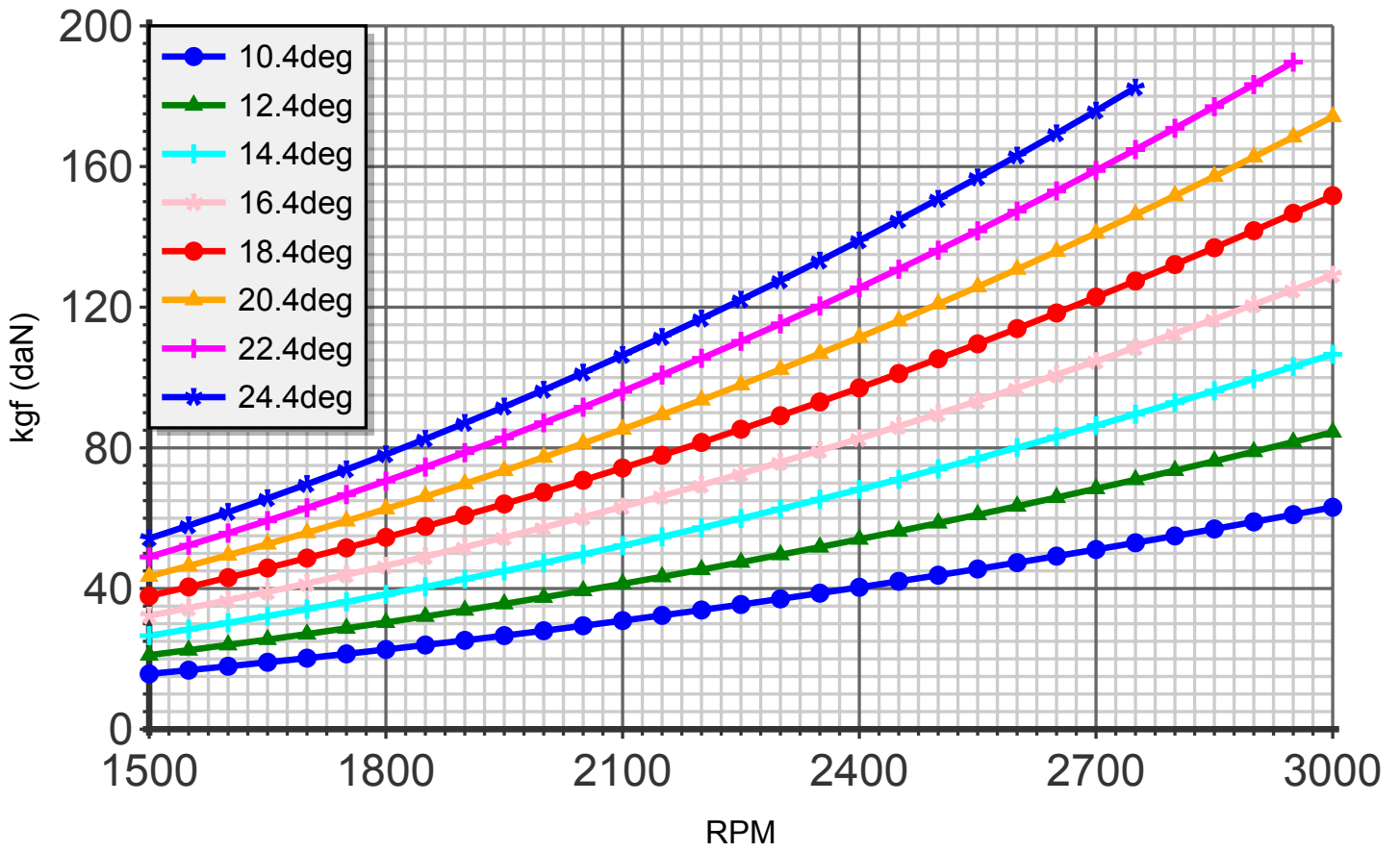
Thrust (blade:3 diameter:150cm R-1300)
