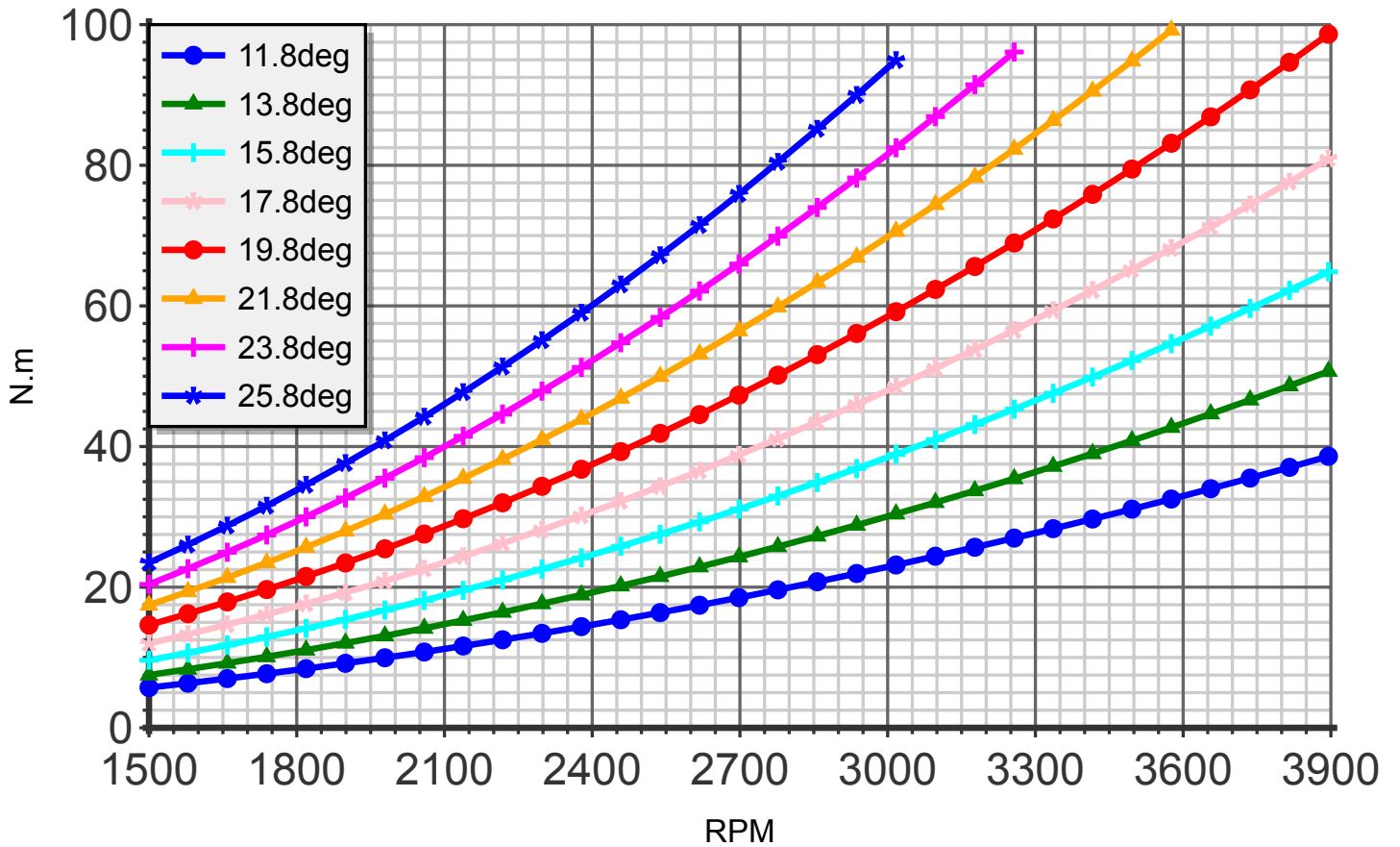
Torque (blade:2 diameter:125cm R-0600)
