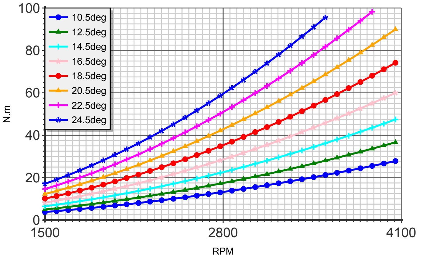
Torque (blade:2 diameter:120cm R-0500)
