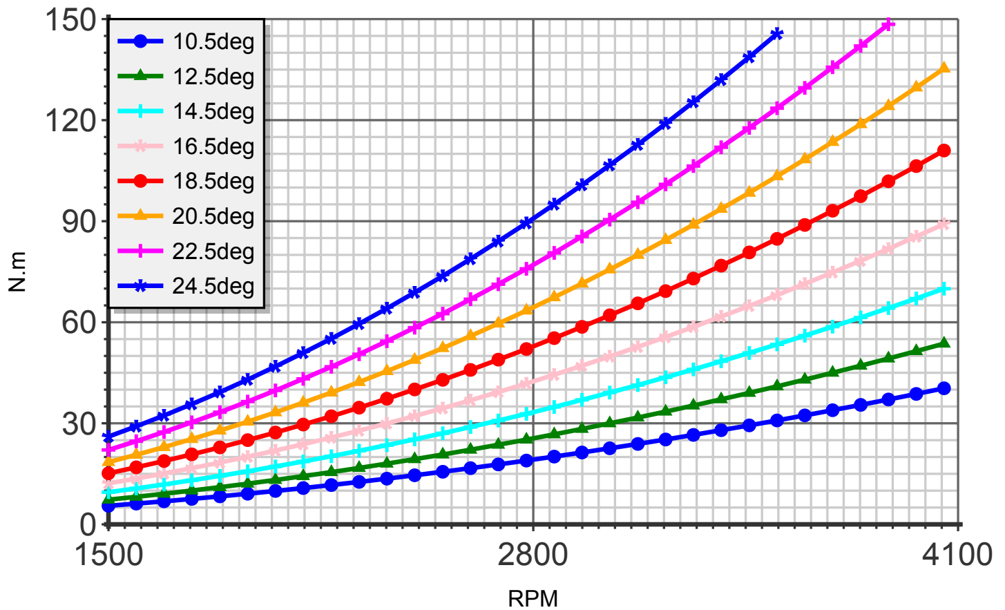
Torque (blade:3 diameter:120cm R-0500)
