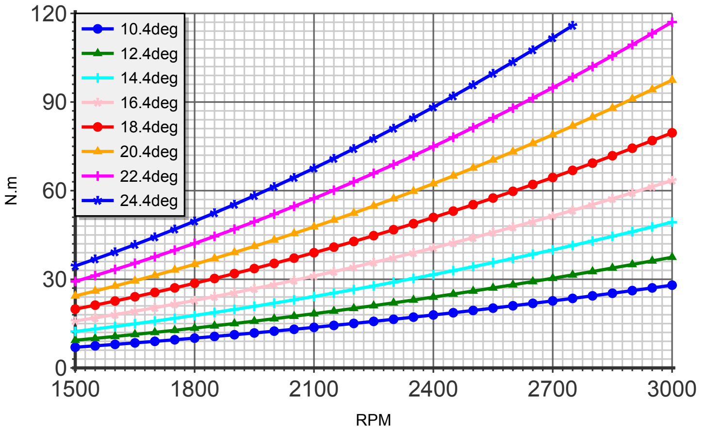
Torque (blade:2 diameter:150cm R-1300)
