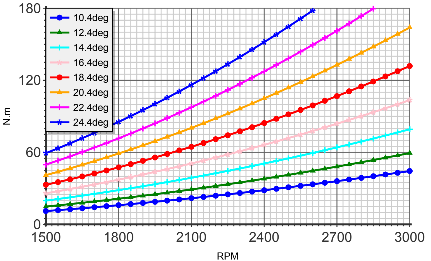
Torque (blade:3 diameter:160cm R-1300)
