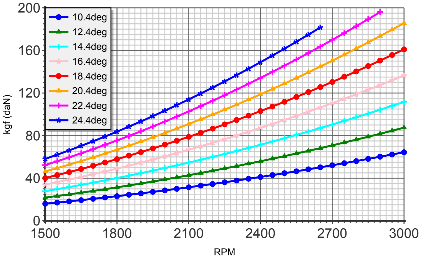
Thrust (blade:3 diameter:155cm R-1300)
