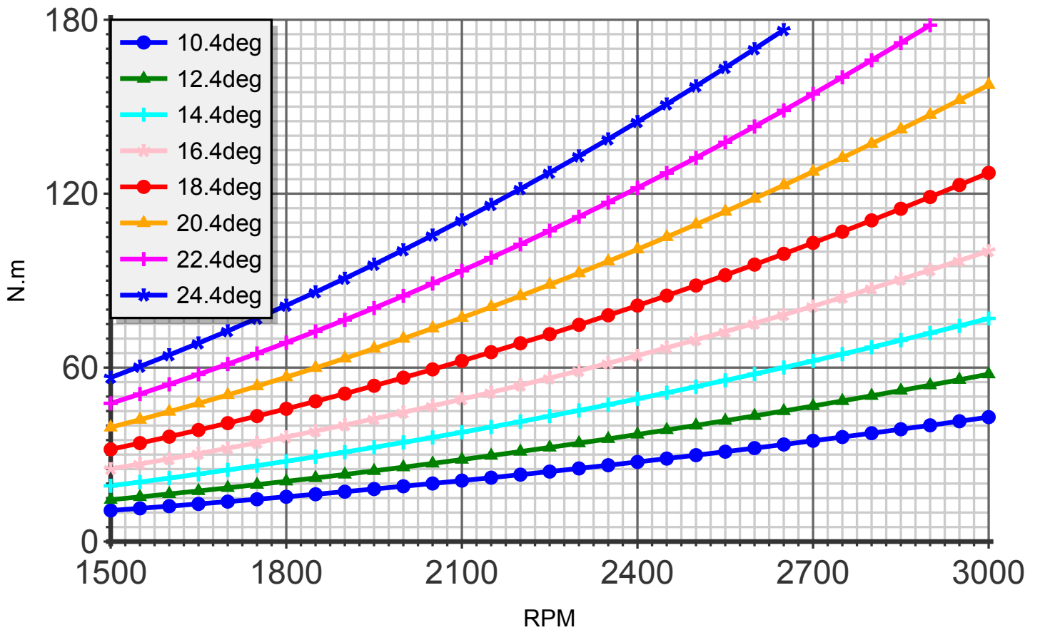
Torque (blade:3 diameter:155cm R-1300)
