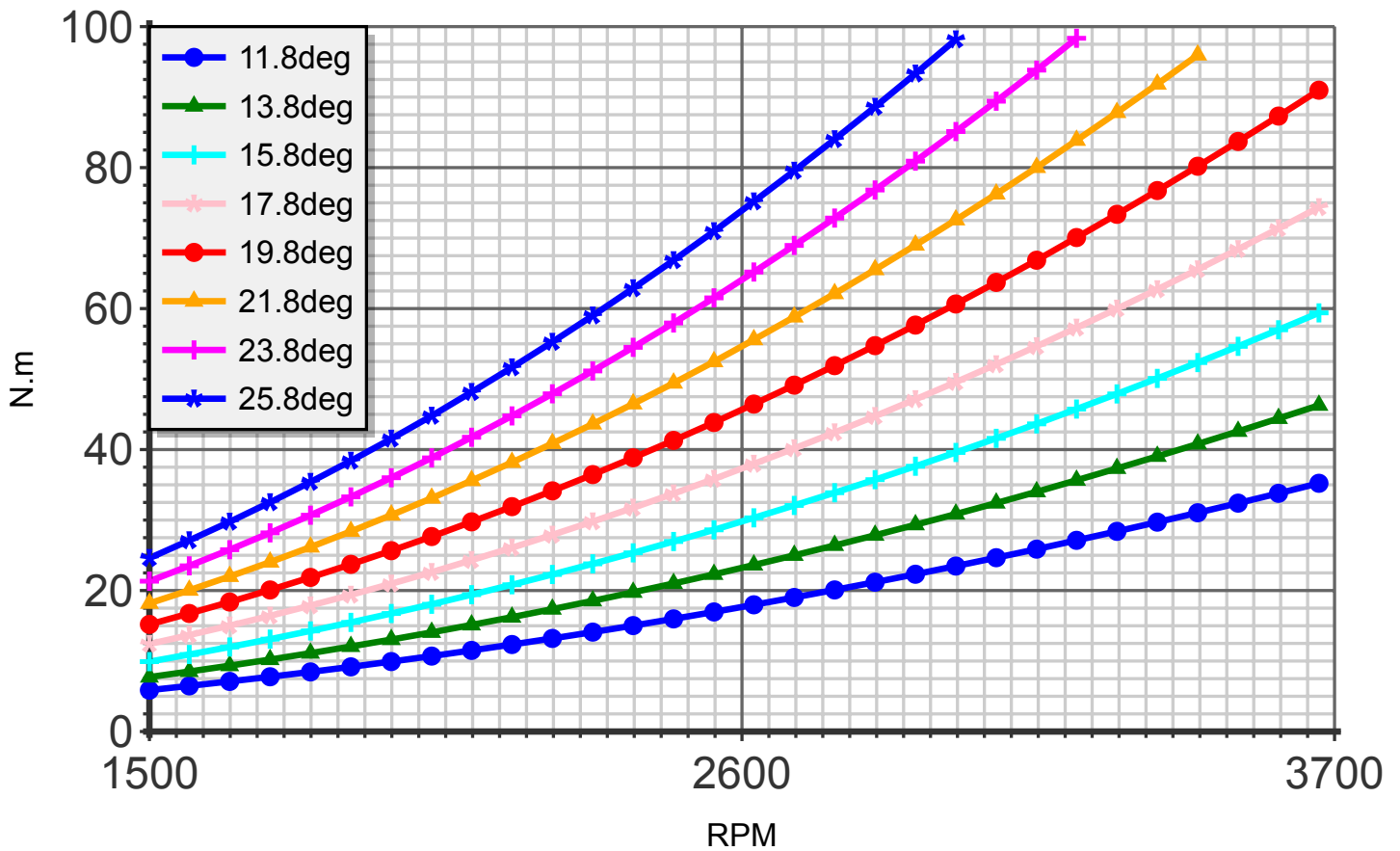
Torque (blade:2 diameter:130cm R-0600)
