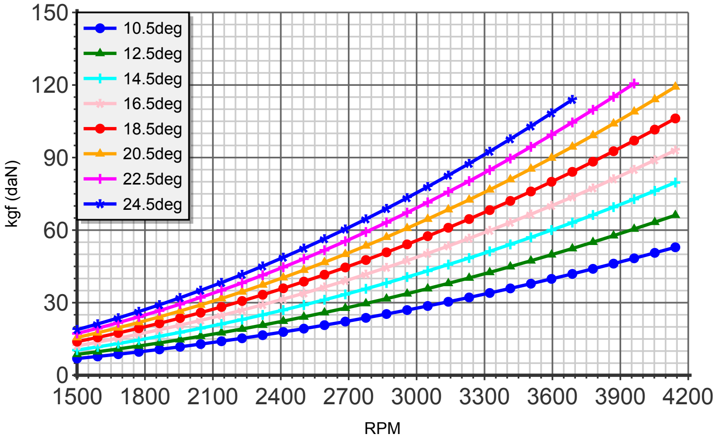
Thrust (blade:2 diameter:115cm R-0500)
