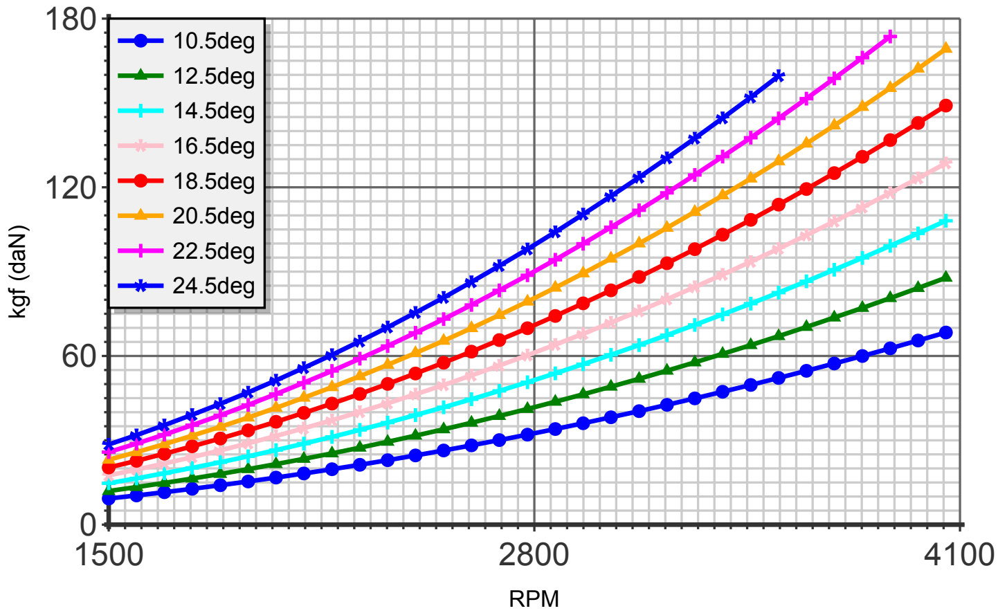
Thrust (blade:3 diameter:120cm R-0500)
