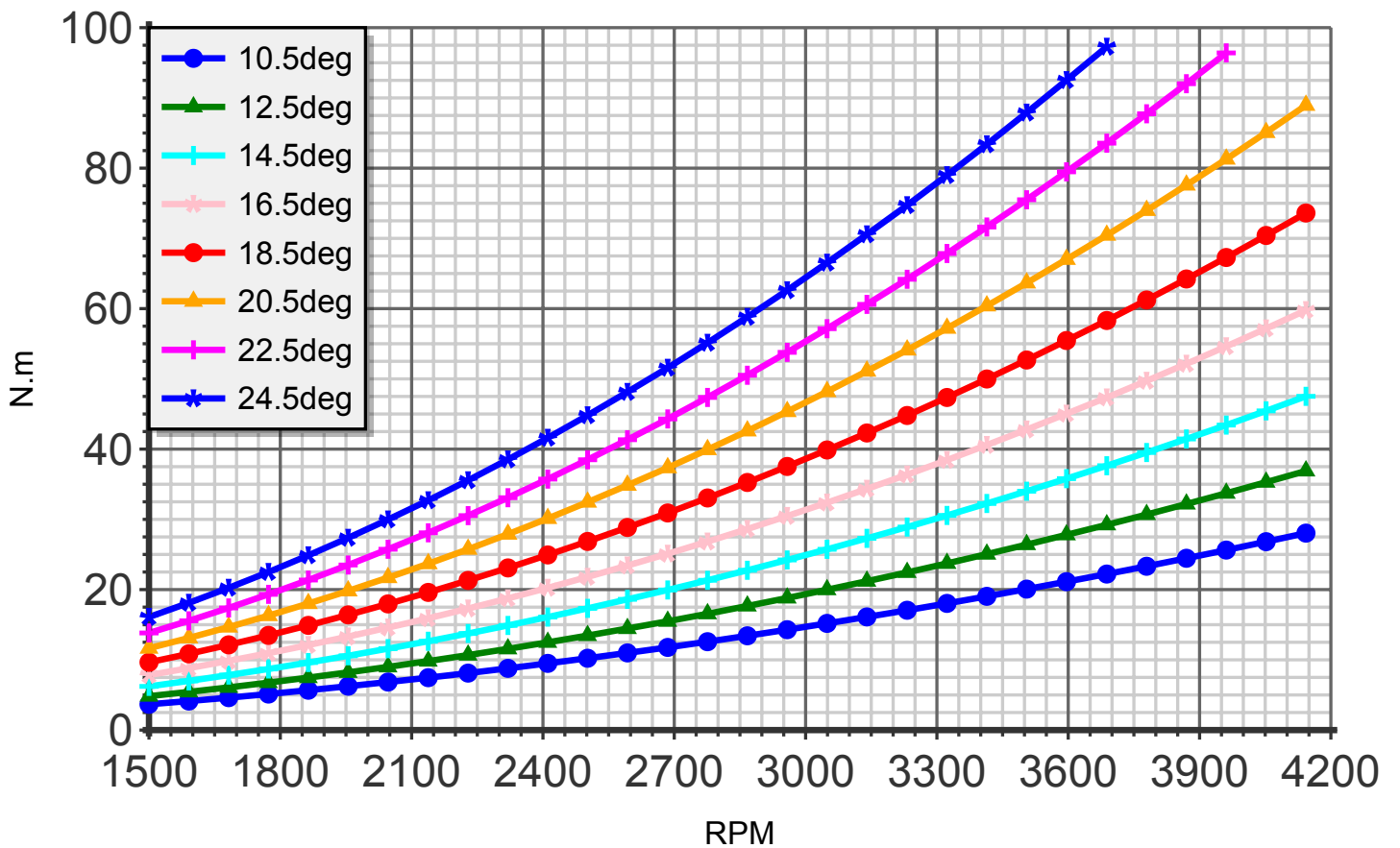
Torque (blade:2 diameter:115cm R-0500)
