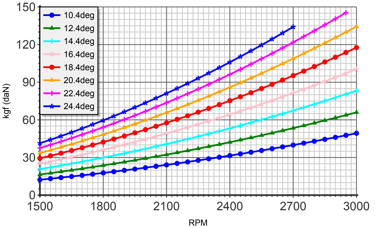
Thrust (blade:2 diameter:155cm R-1300)
