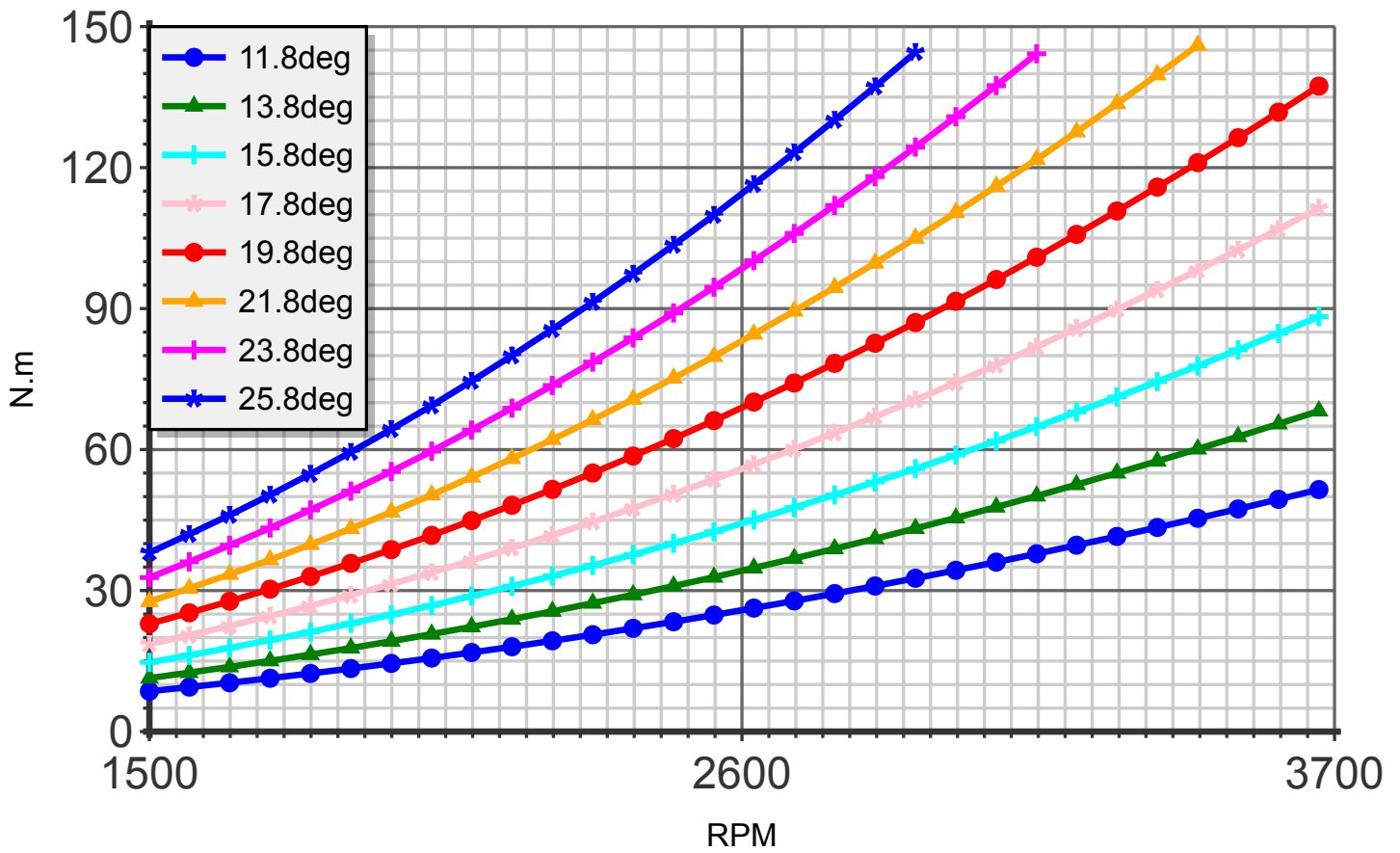
Torque (blade:3 diameter:130cm R-0600)
