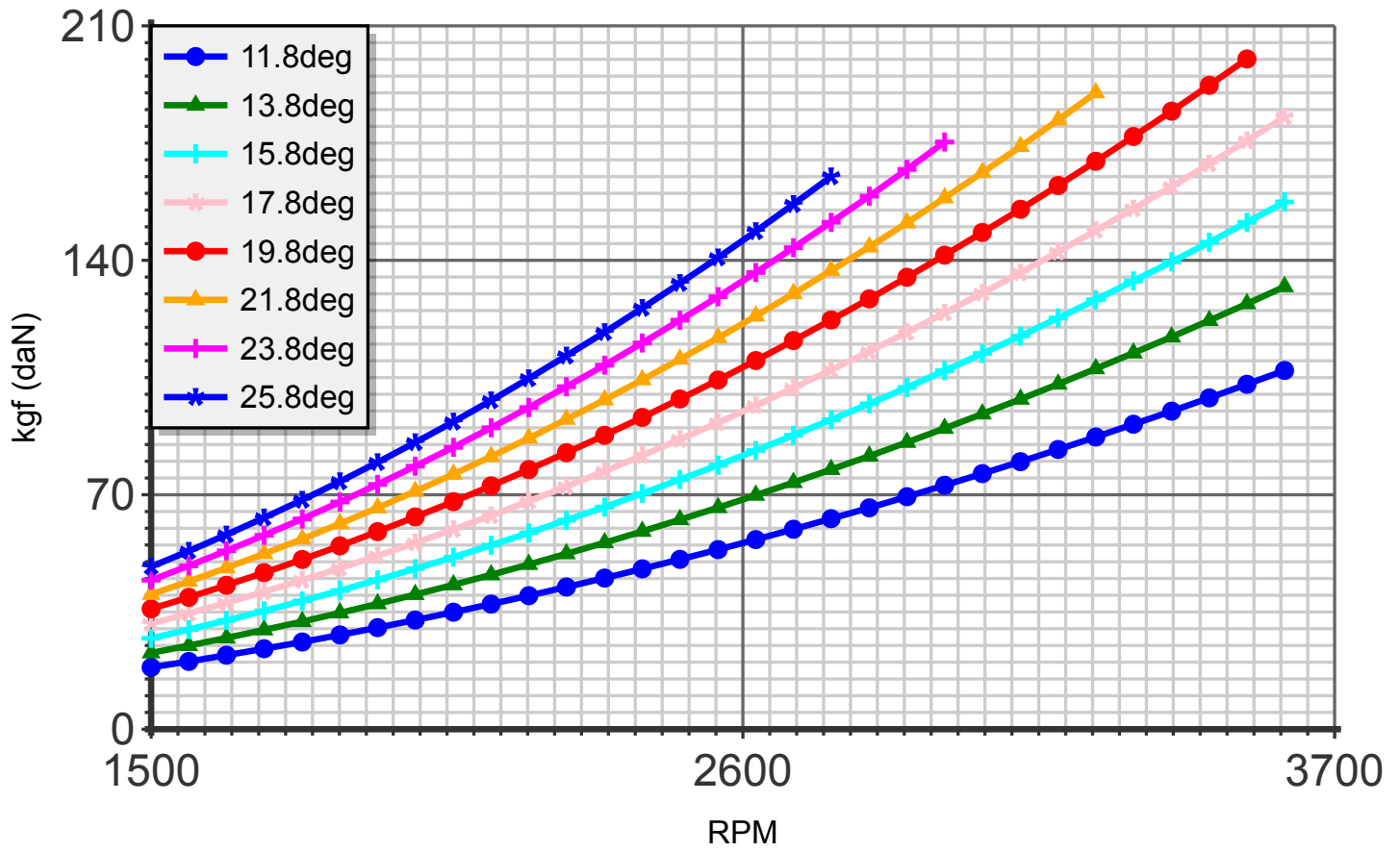
Thrust (blade:3 diameter:135cm R-1100)
