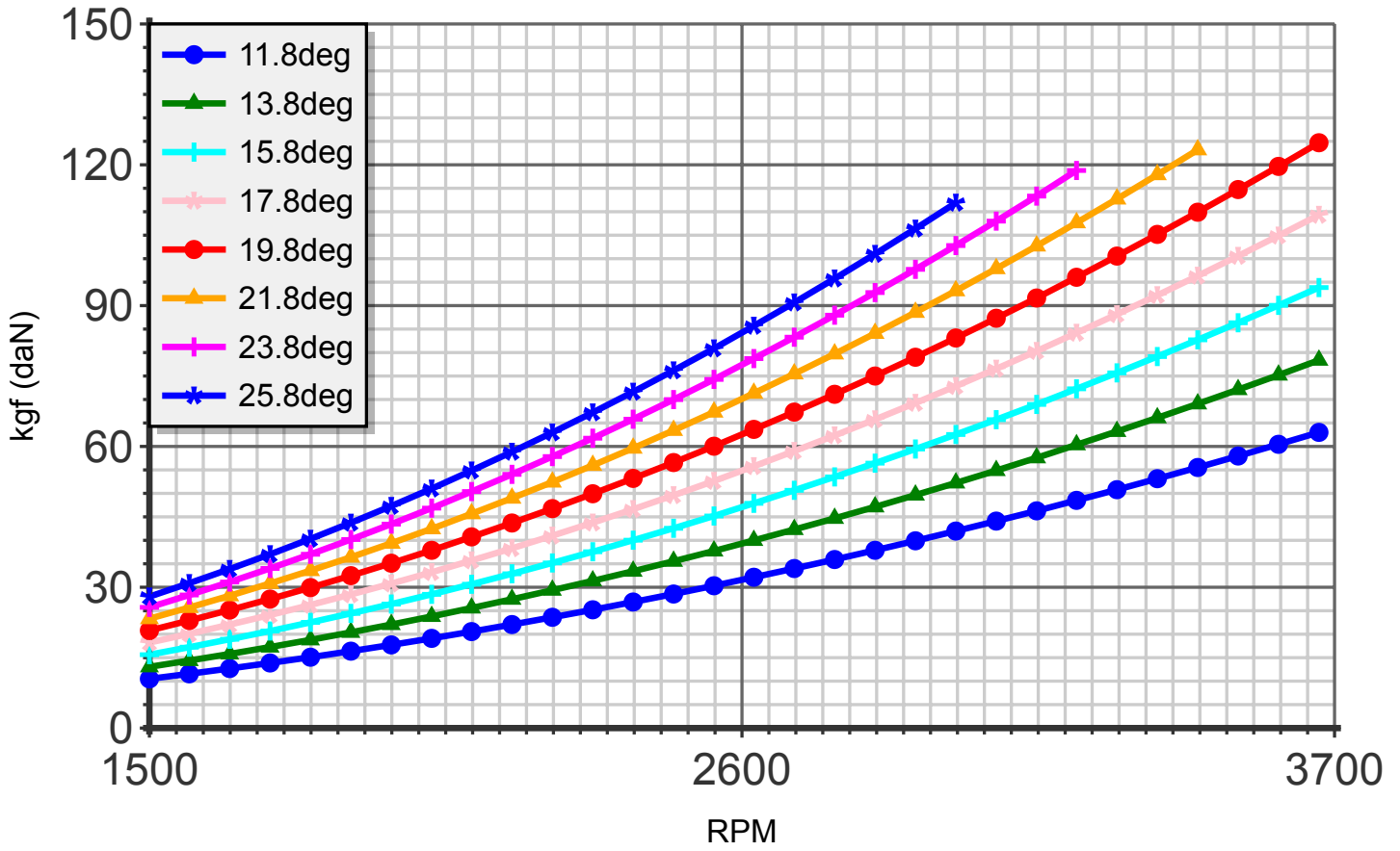
Thrust (blade:2 diameter:130cm R-0600)
