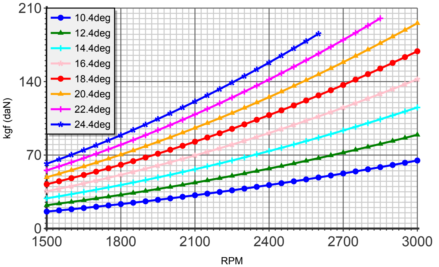
Thrust (blade:3 diameter:160cm R-1300)
