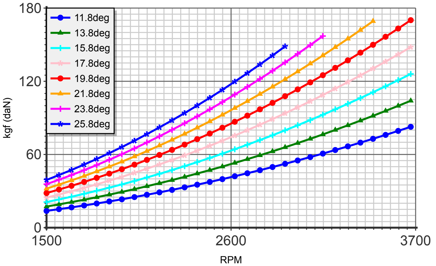
Thrust (blade:3 diameter:130cm R-0600)
