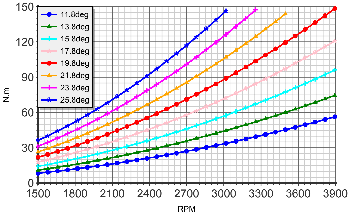
Torque (blade:3 diameter:125cm R-0600)
