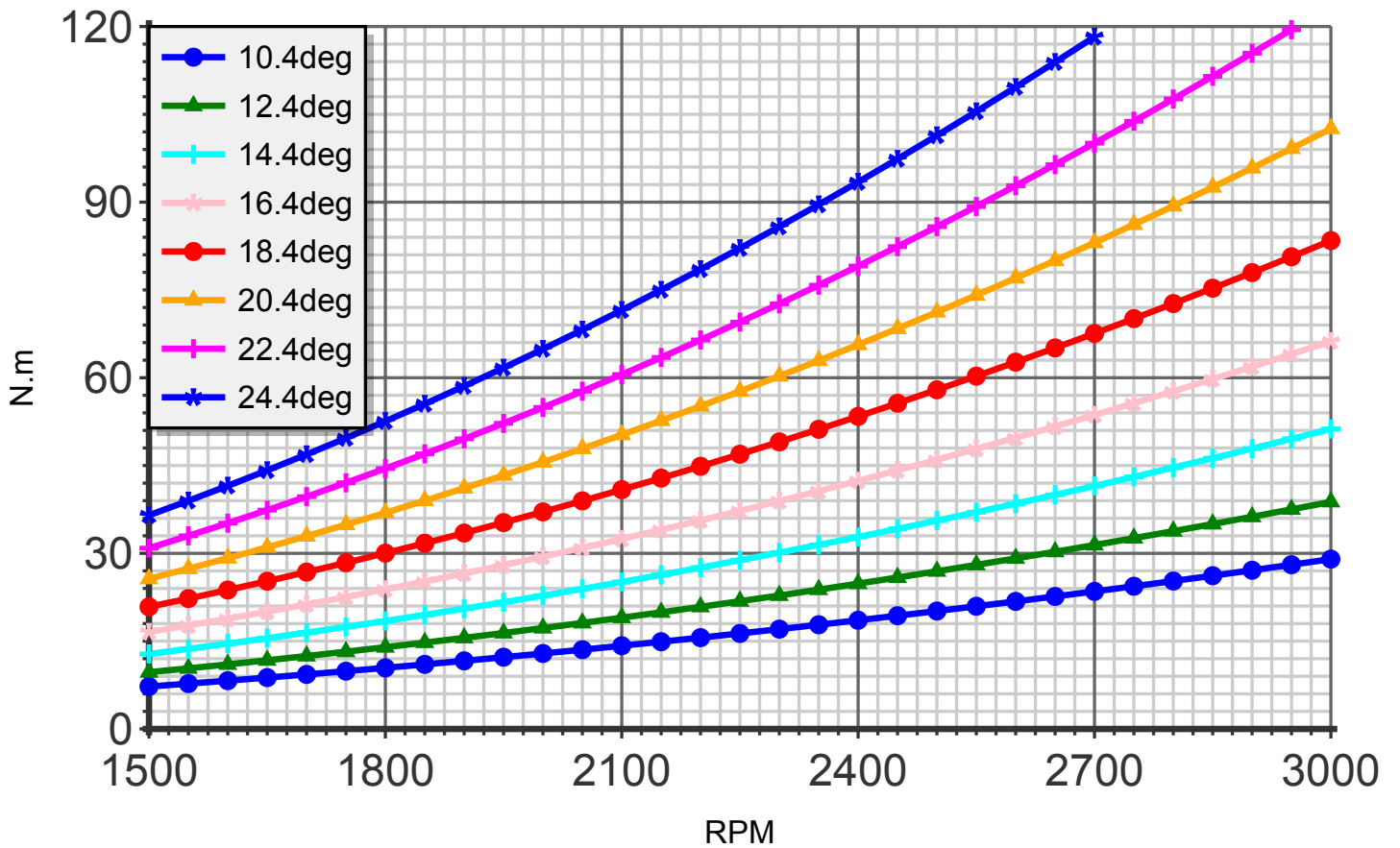
Torque (blade:2 diameter:155cm R-1300)
