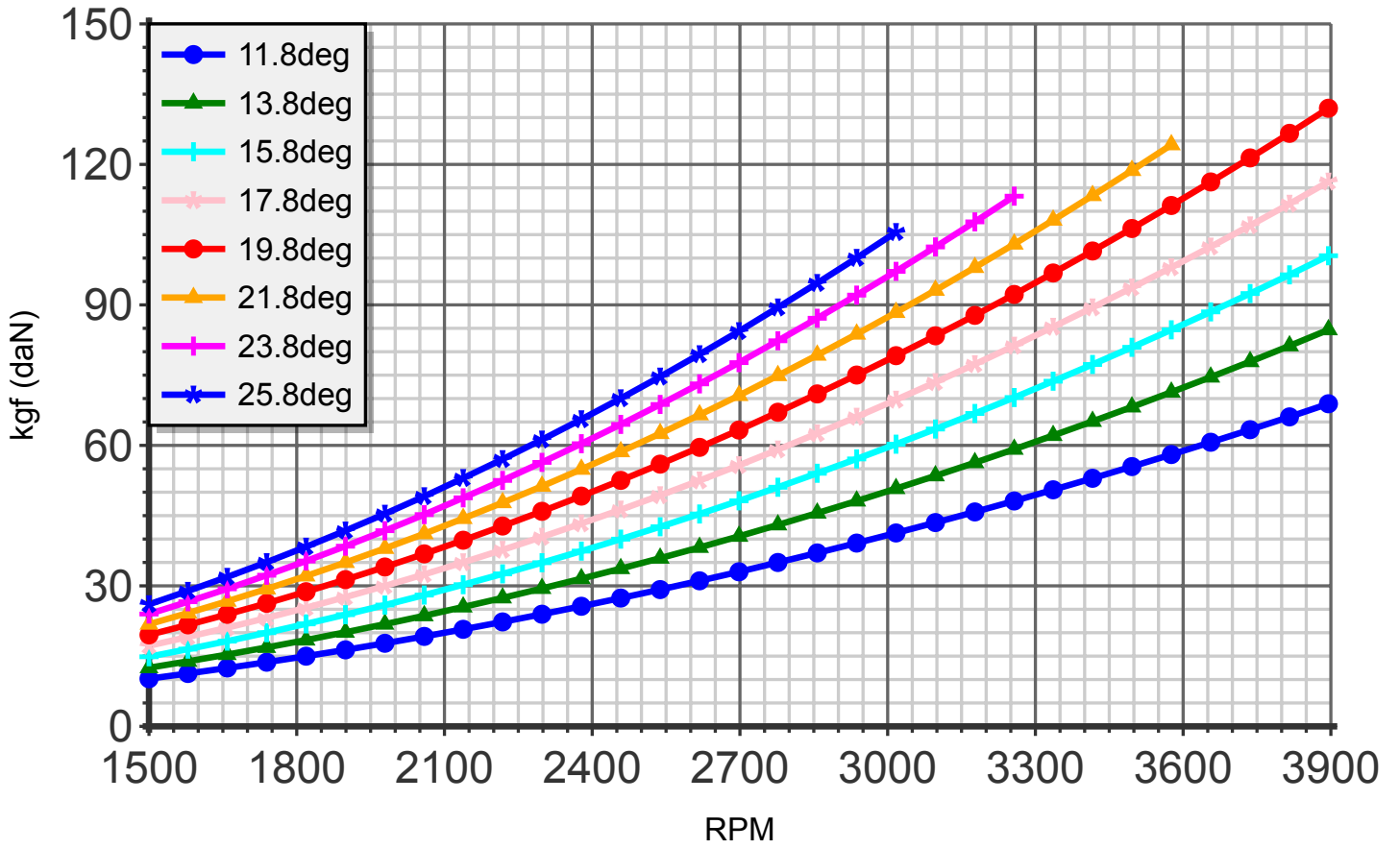
Thrust (blade:2 diameter:125cm R-0600)
