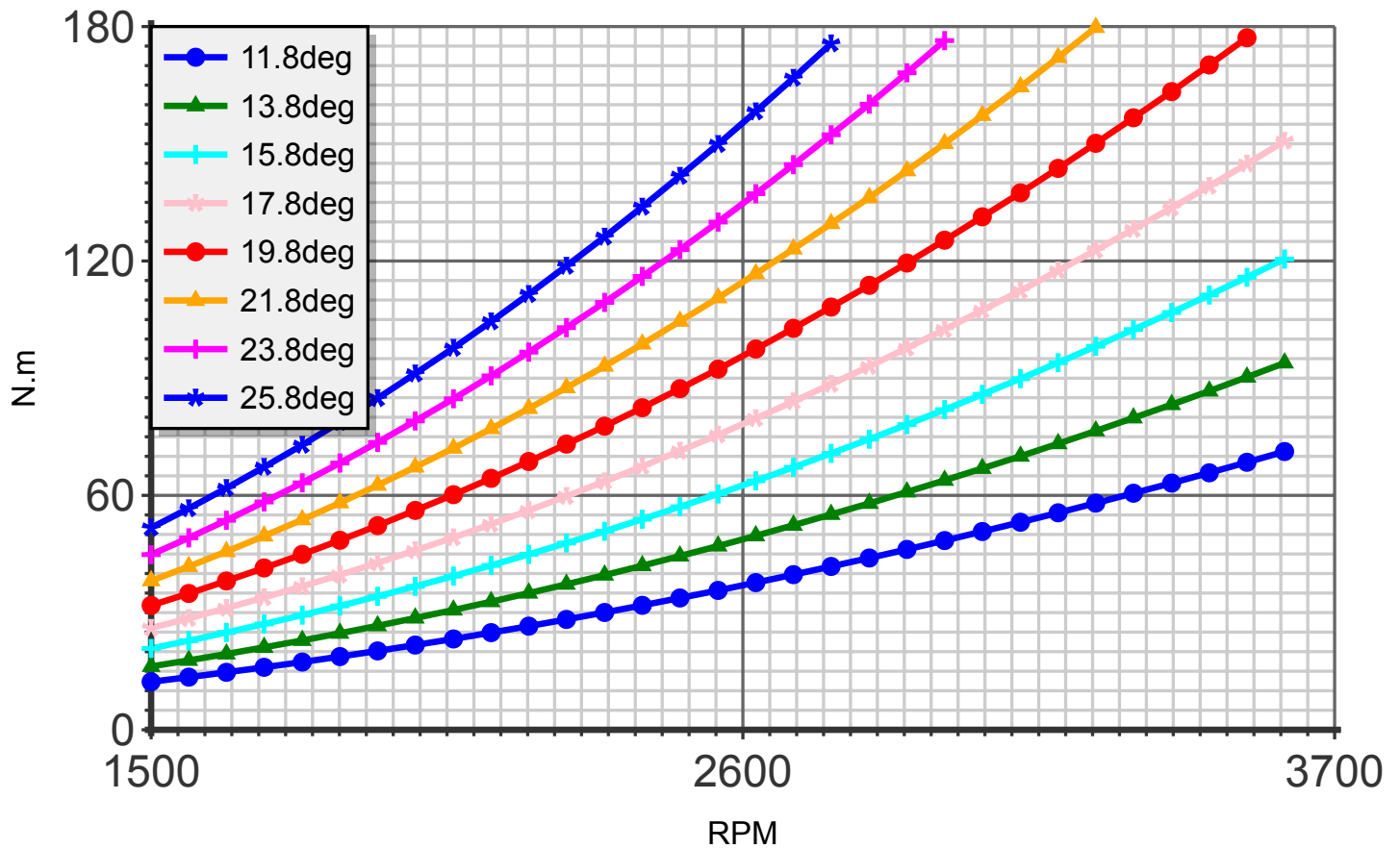
Torque (blade:3 diameter:135cm R-1100)
