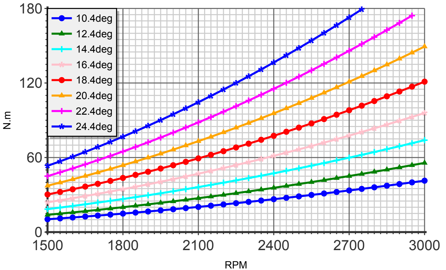
Torque (blade:3 diameter:150cm R-1300)
