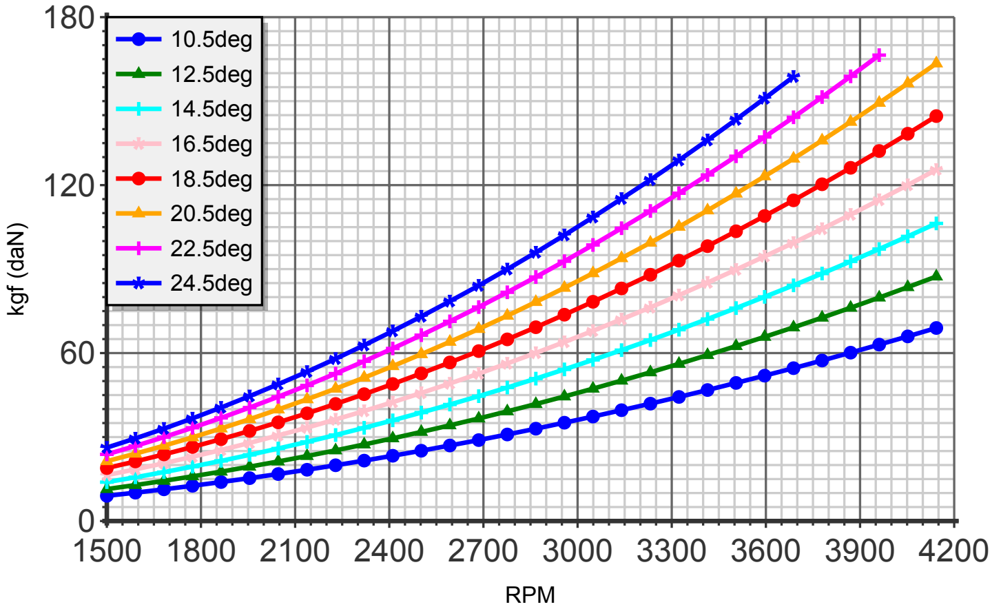
Thrust (blade:3 diameter:115cm R-0500)
