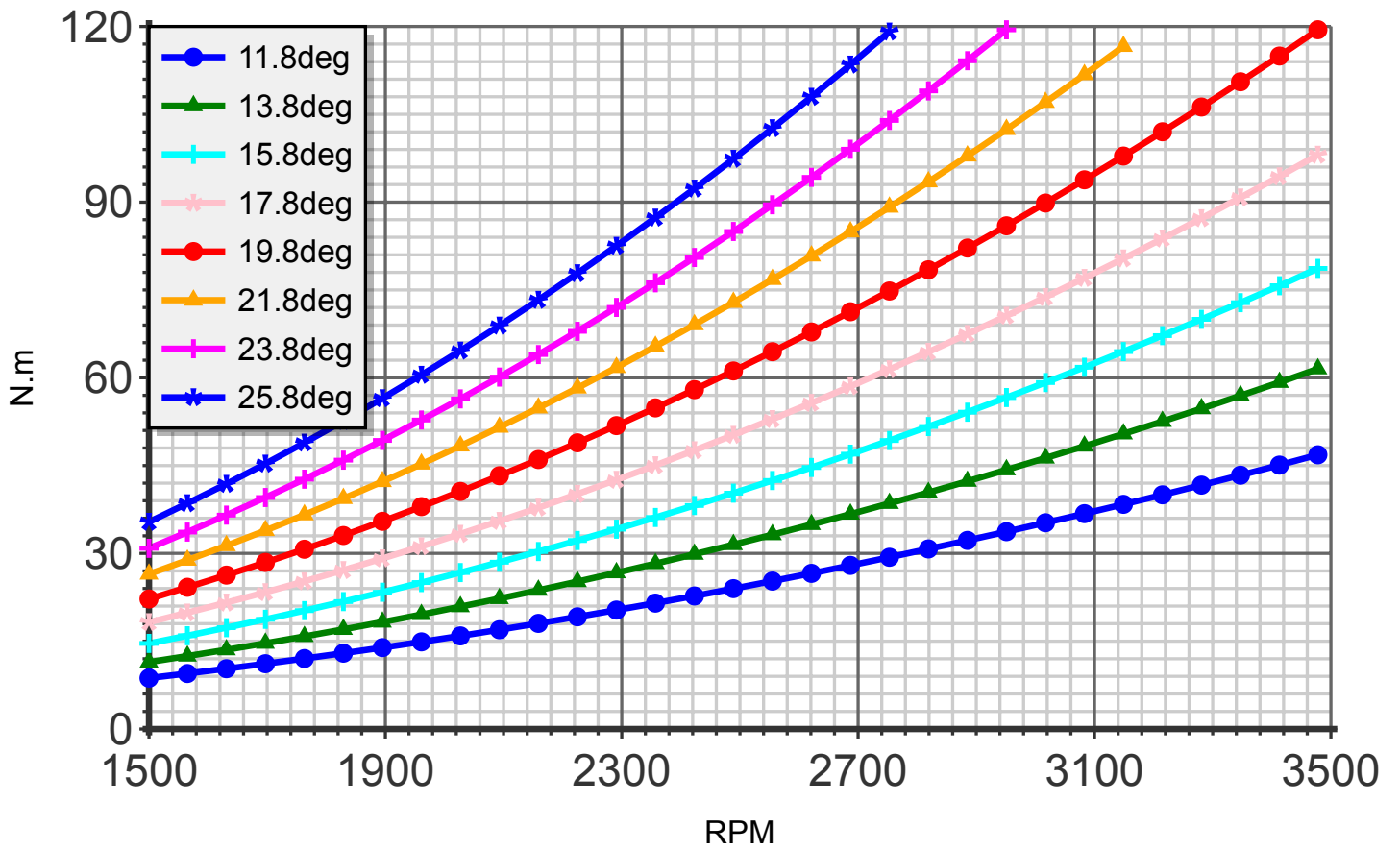
Torque (blade:2 diameter:140cm R-1100)
