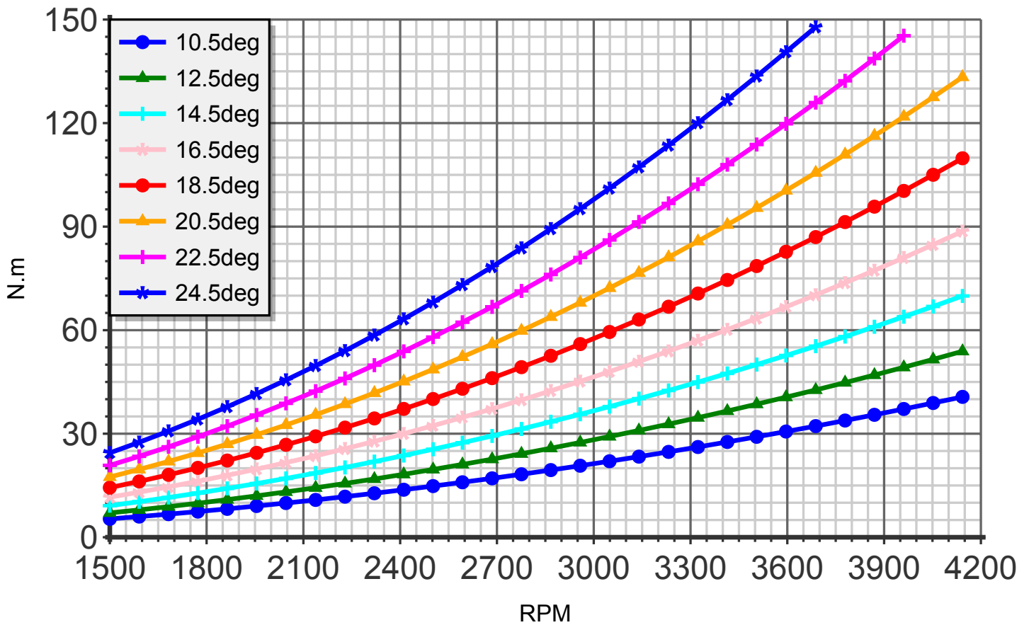
Torque (blade:3 diameter:115cm R-0500)
