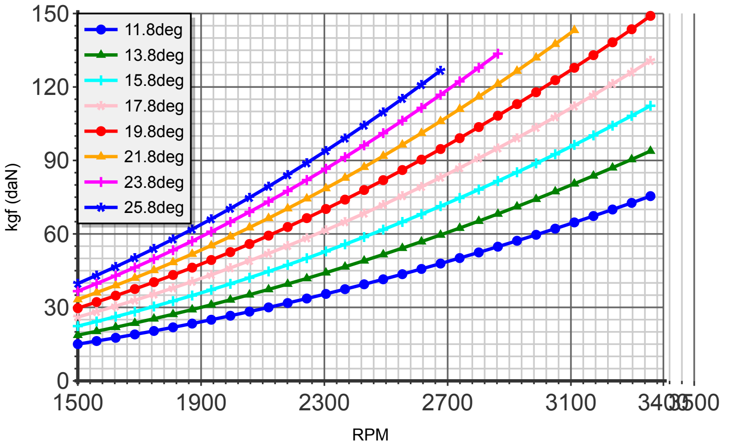
Thrust (blade:2 diameter:145cm R-1100)
