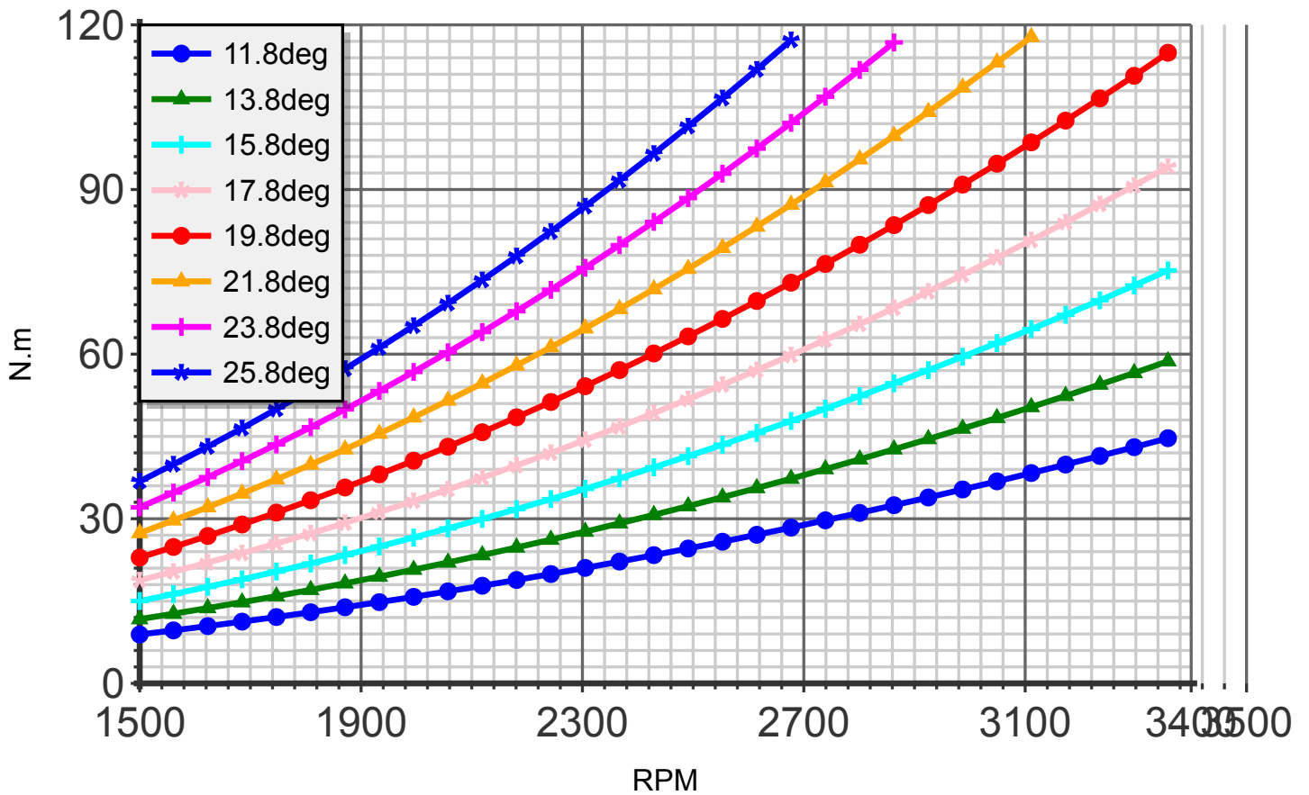
Torque (blade:2 diameter:145cm R-1100)
