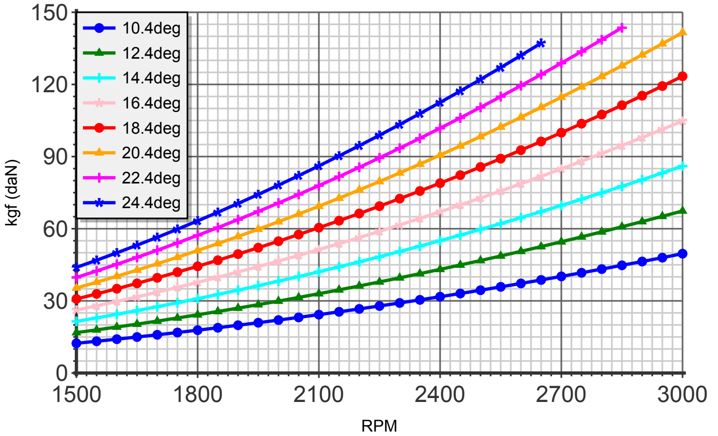
Thrust (blade:2 diameter:160cm R-1300)
