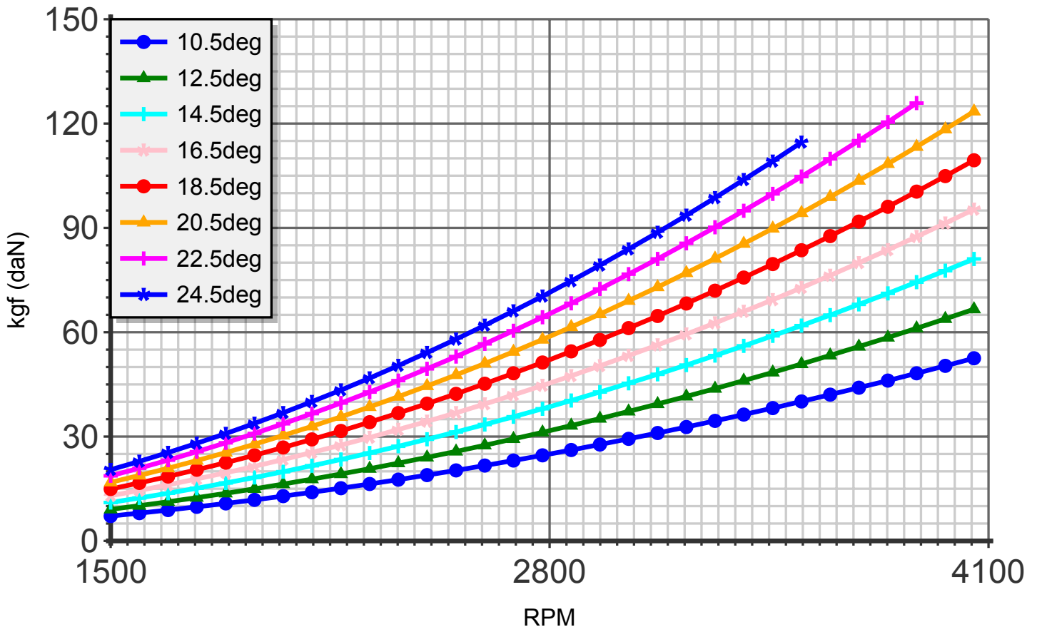
Thrust (blade:2 diameter:120cm R-0500)
