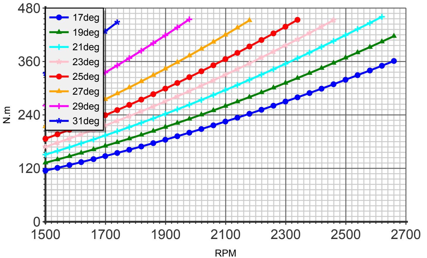
Torque (blade:3 diameter:185cm C4)
