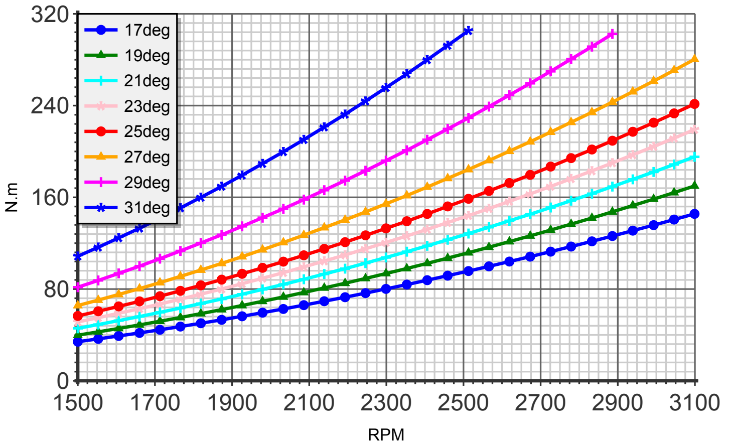
Torque (blade:2 diameter:160cm C4)
