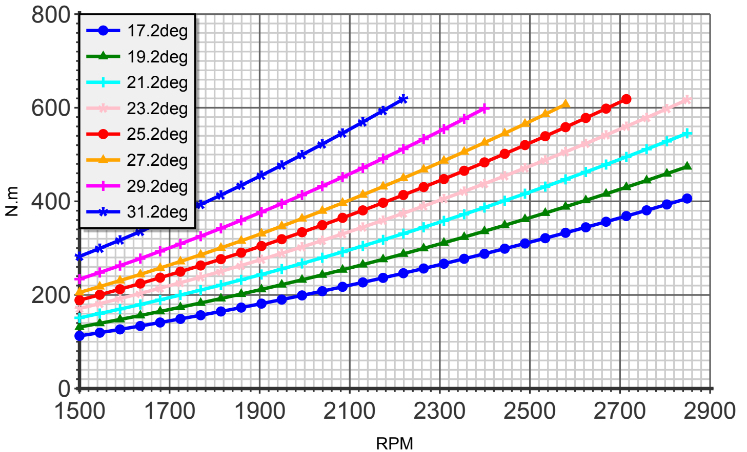
Torque (blade:4 diameter:174cm C4)
