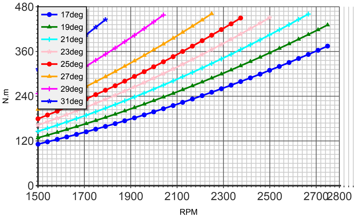
Torque (blade:3 diameter:180cm C4)
