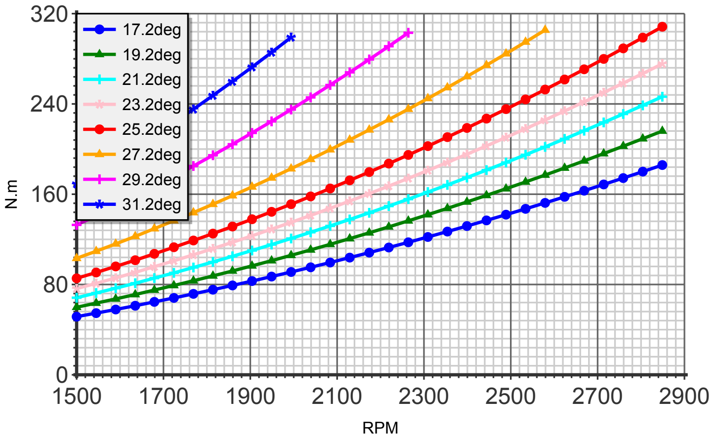
Torque (blade:2 diameter:175cm C4)
