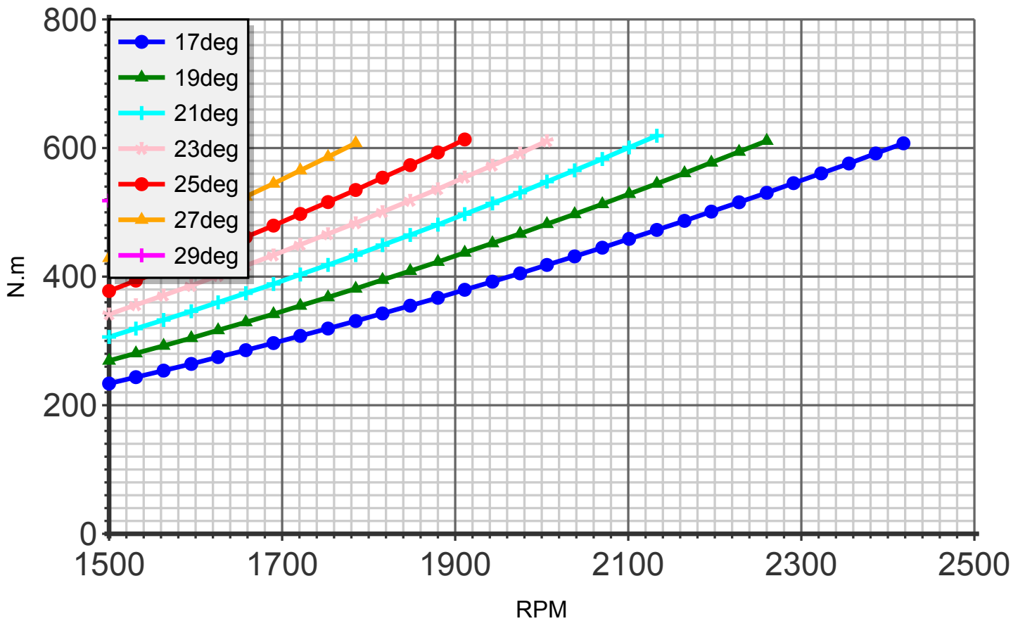
Torque (blade:4 diameter:203cm C4)
