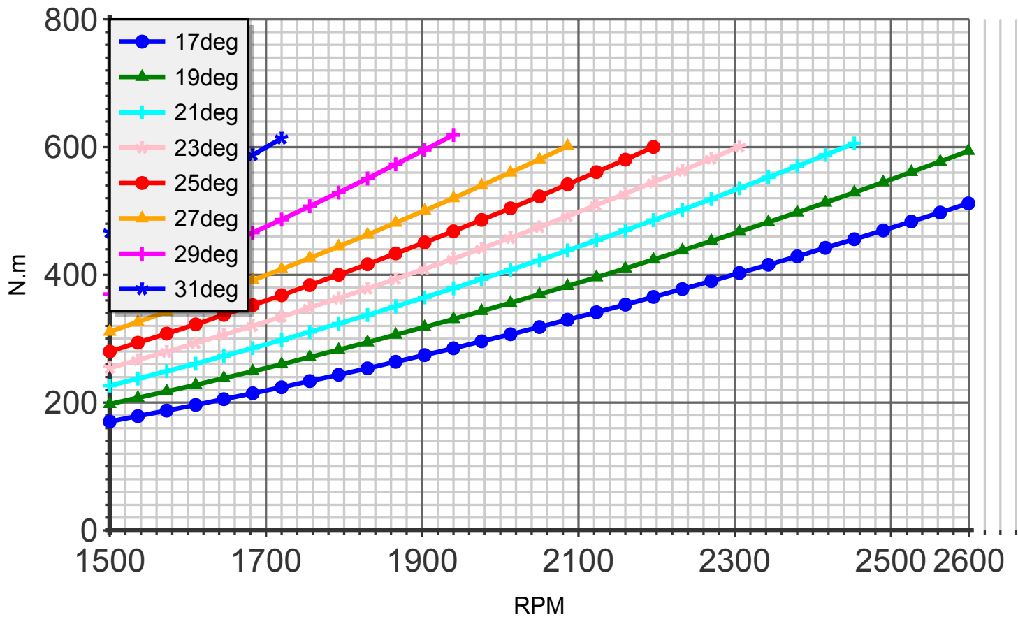
Torque (blade:4 diameter:192cm C4)
