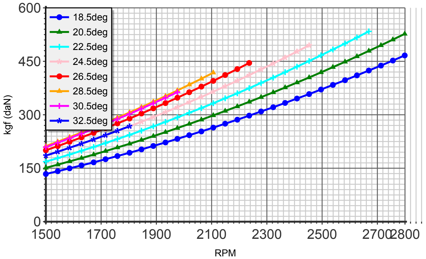
Thrust (blade:5 diameter:179cm C8)
