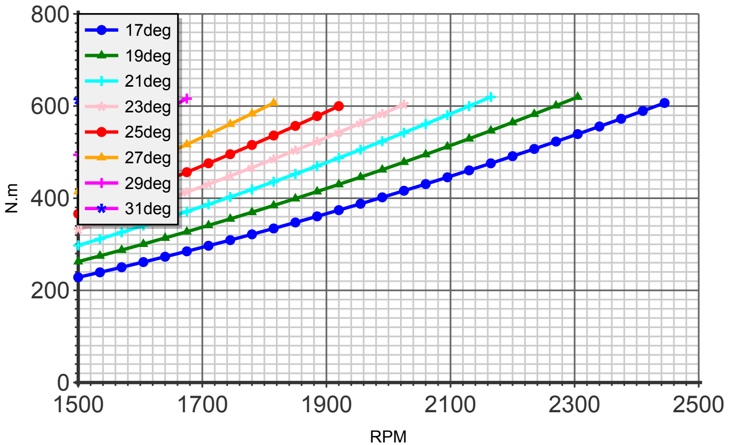
Torque (blade:4 diameter:198cm C4)
