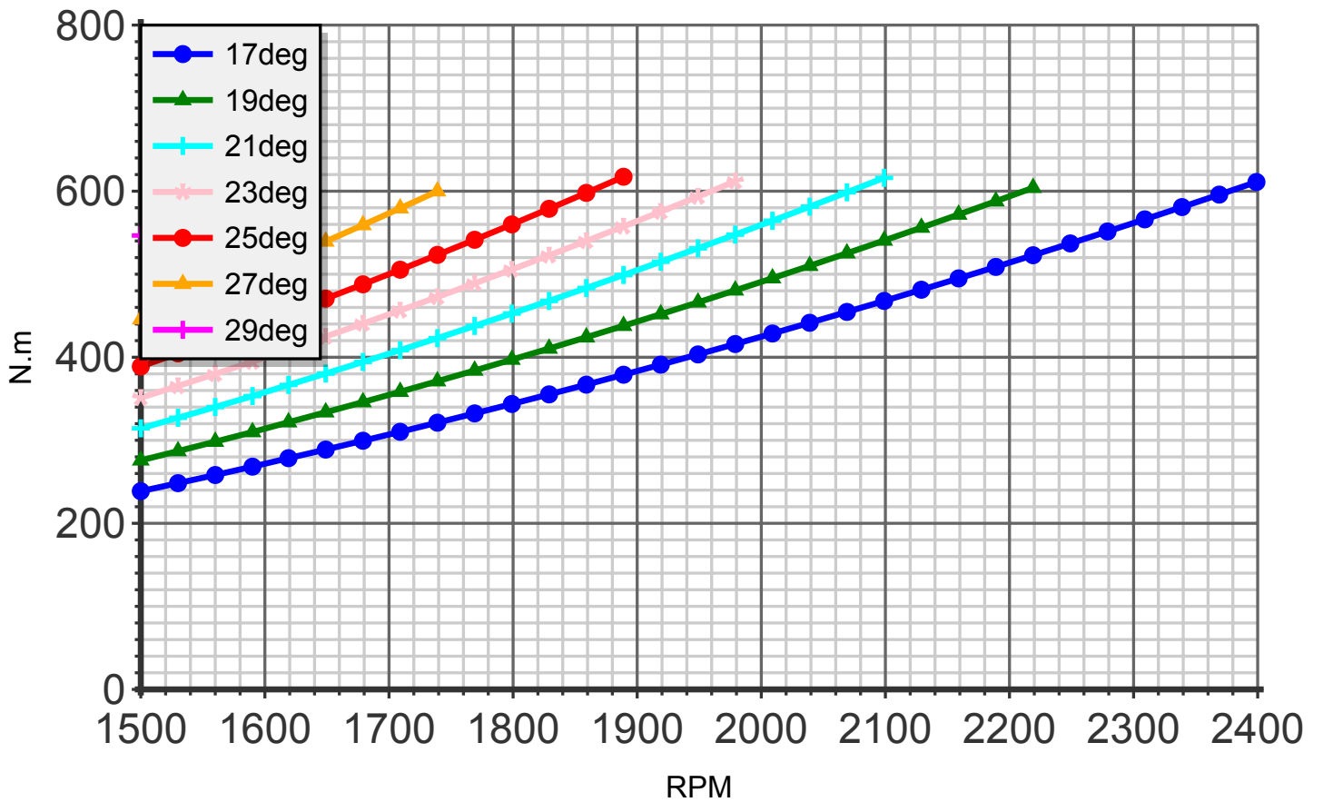
Torque (blade:4 diameter:208cm C4)
