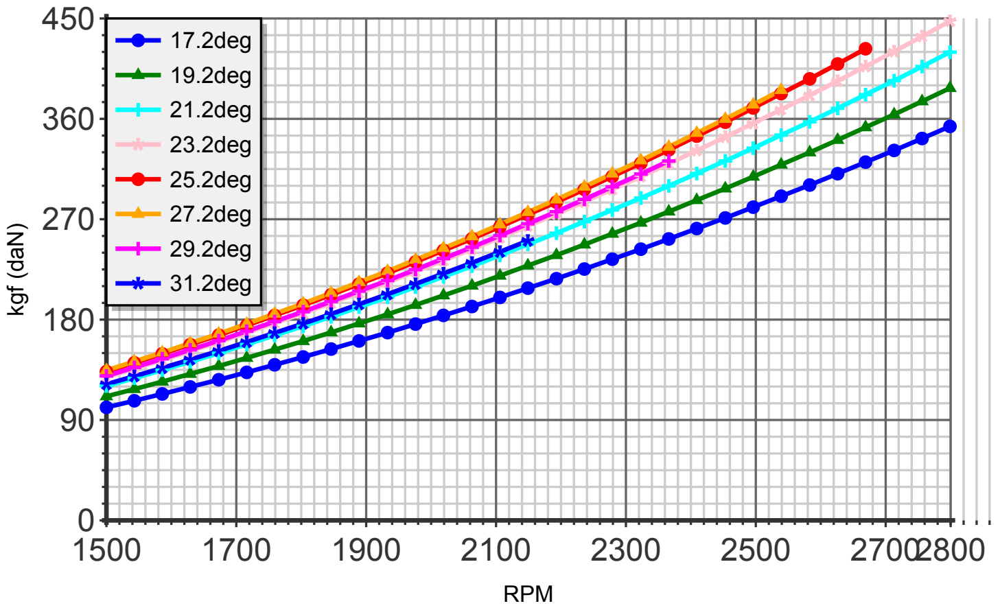
Thrust (blade:4 diameter:177cm C4)
