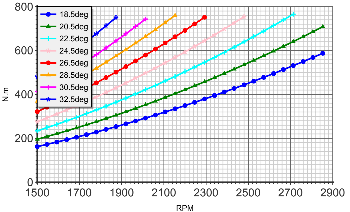
Torque (blade:5 diameter:174cm C8)
