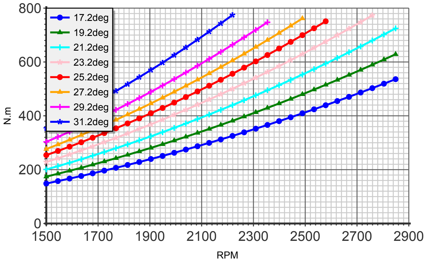
Torque (blade:5 diameter:176cm C4)
