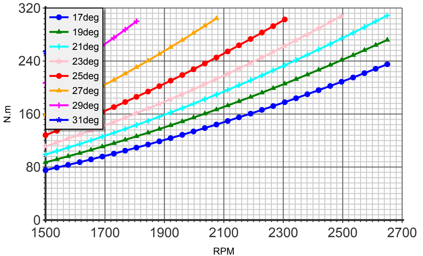
Torque (blade:2 diameter:190cm C4)
