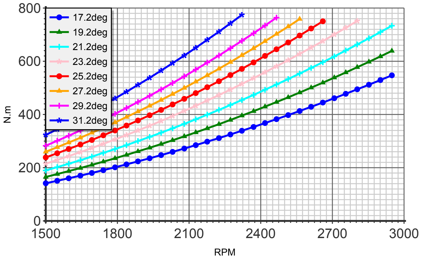
Torque (blade:5 diameter:169cm C4)
