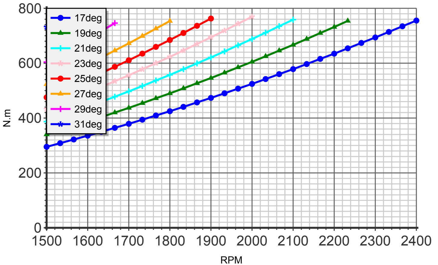
Torque (blade:5 diameter:199cm C4)
