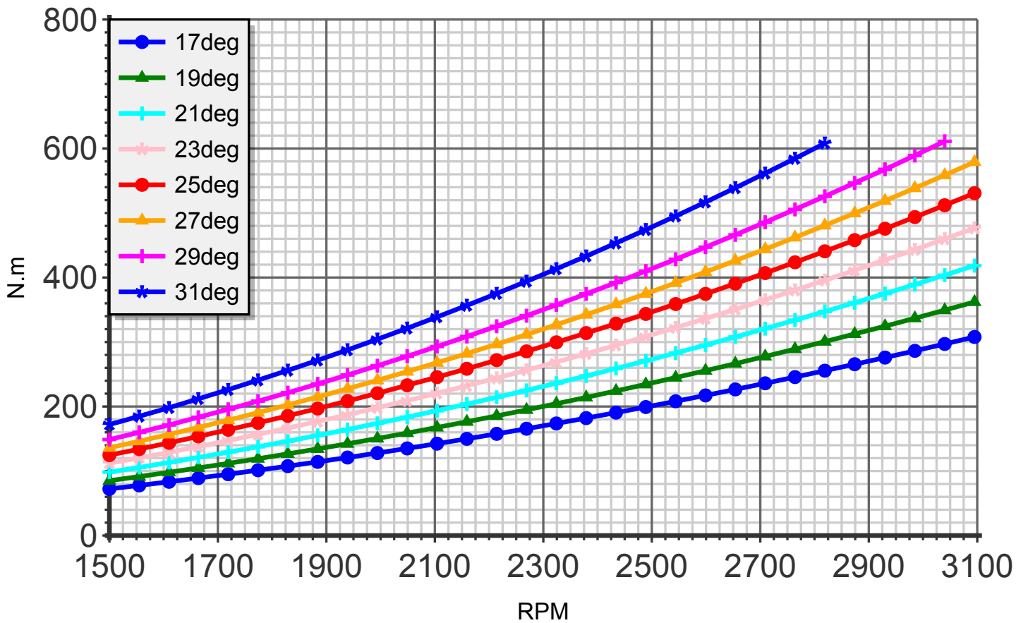
Torque (blade:4 diameter:157cm C4)
