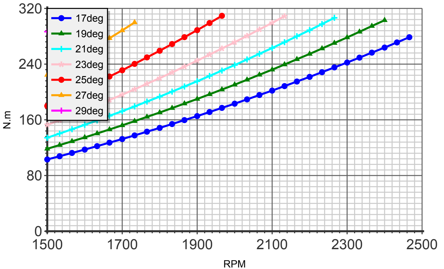
Torque (blade:2 diameter:200cm C4)
