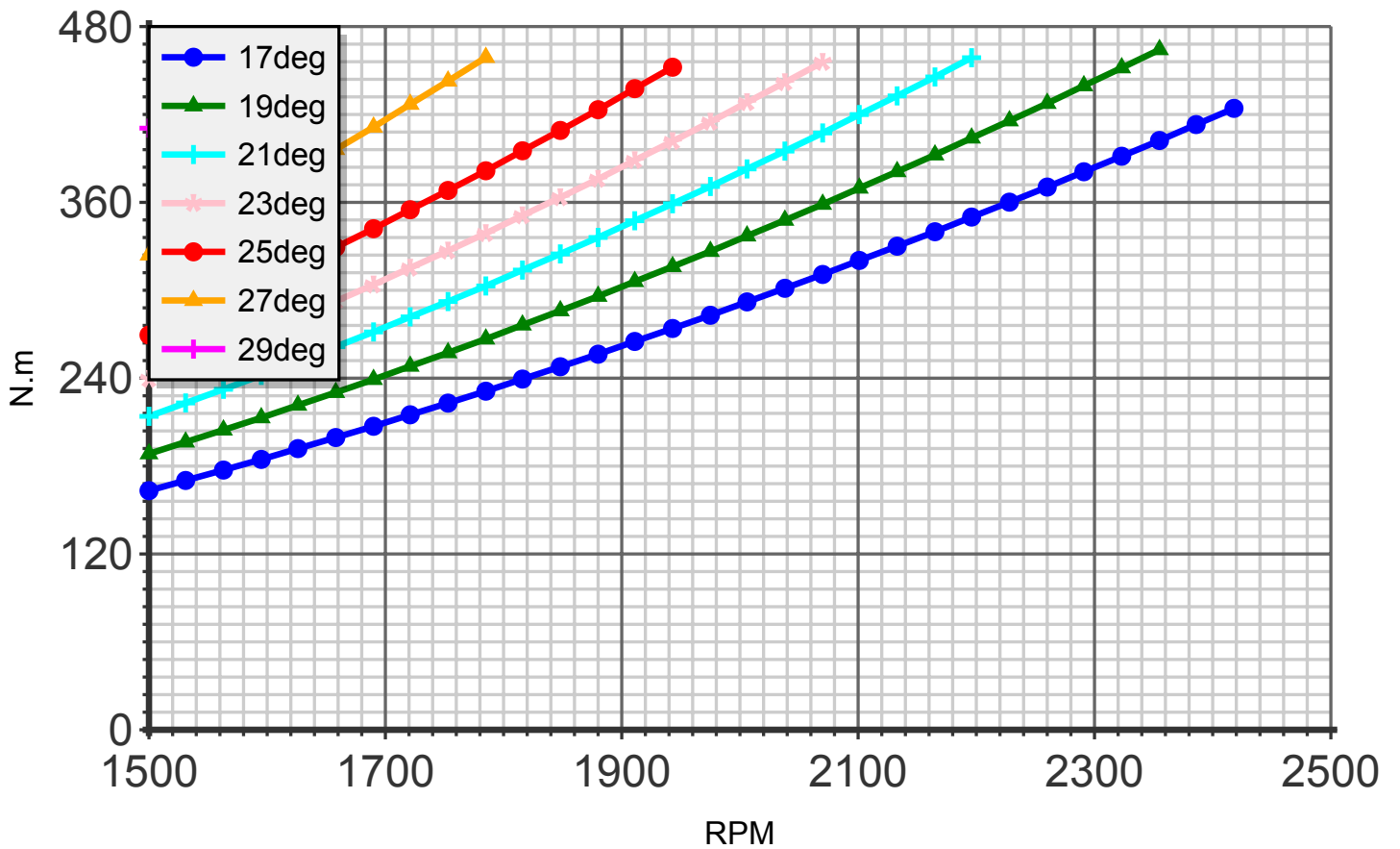
Torque (blade:3 diameter:205cm C4)
