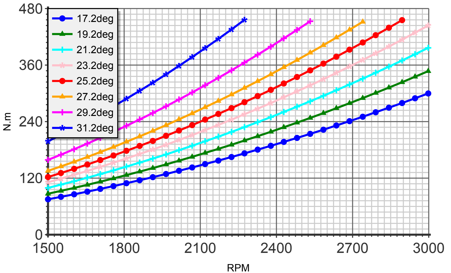
Torque (blade:3 diameter:165cm C4)
