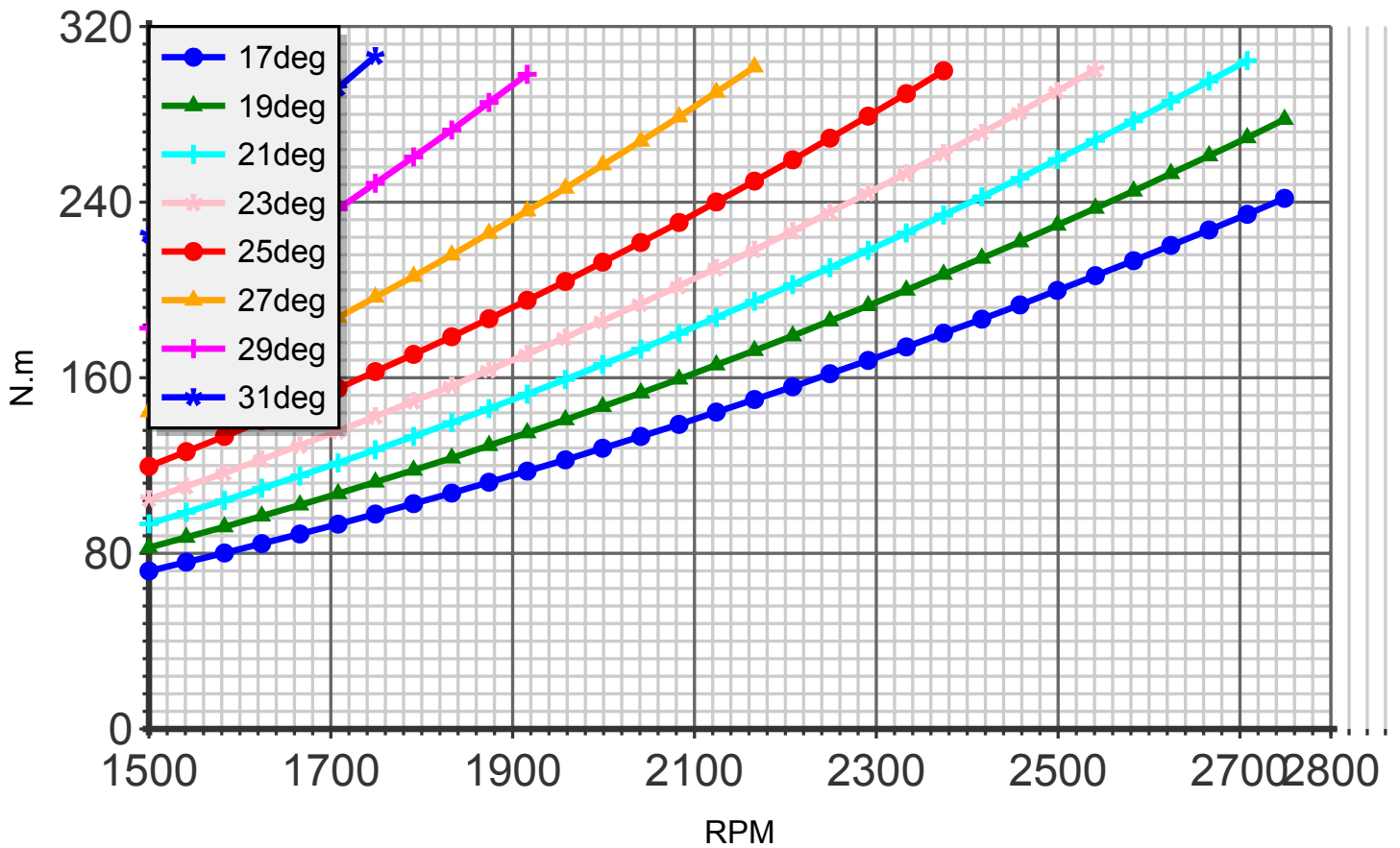
Torque (blade:2 diameter:180cm C4)
