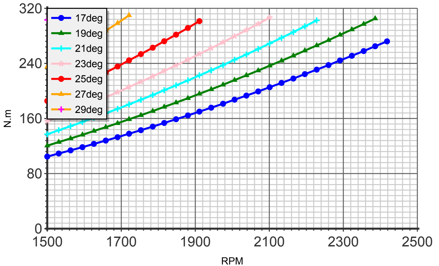
Torque (blade:2 diameter:205cm C4)
