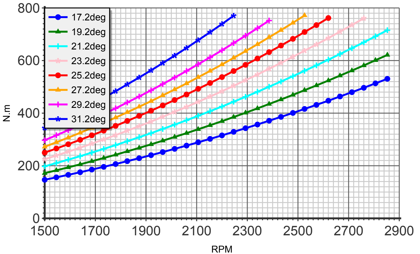
Torque (blade:5 diameter:174cm C4)
