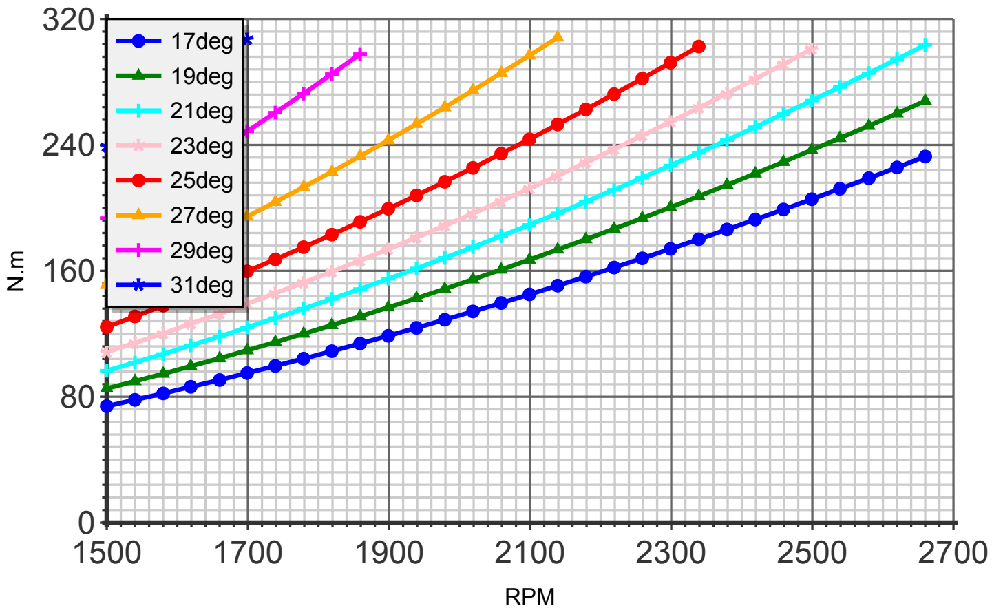
Torque (blade:2 diameter:185cm C4)
