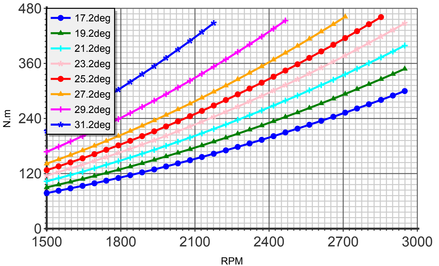
Torque (blade:3 diameter:170cm C4)
