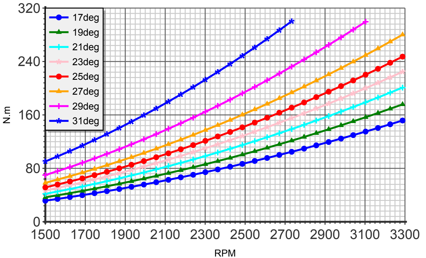
Torque (blade:2 diameter:150cm C4)
