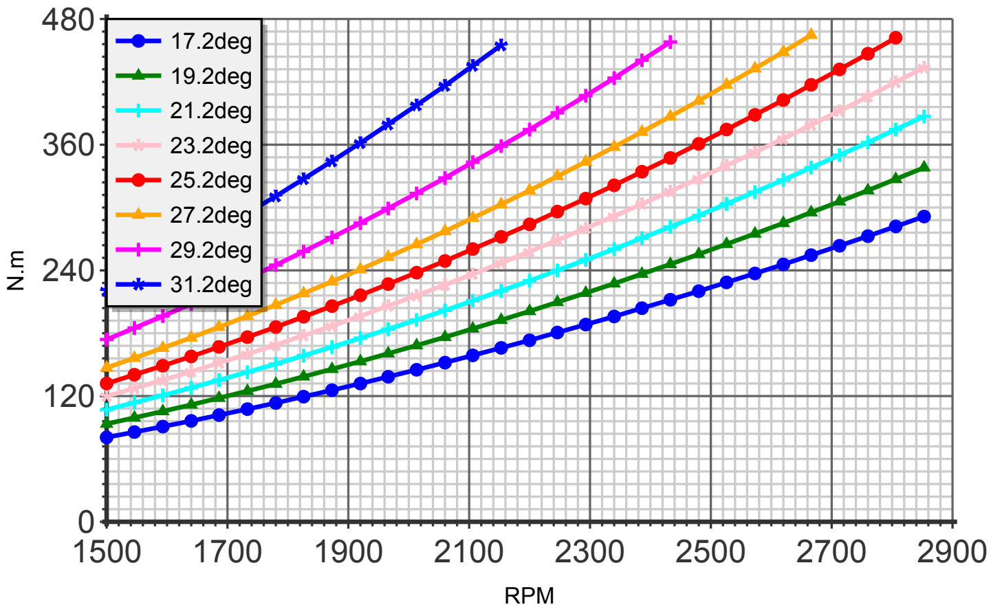
Torque (blade:3 diameter:172cm C4)
