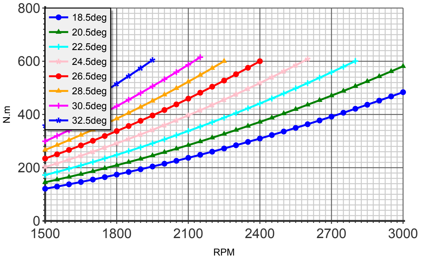
Torque (blade:4 diameter:167cm C8)
