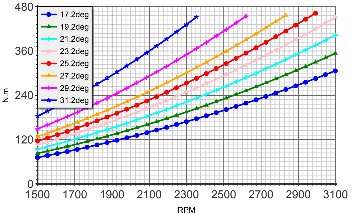
Torque (blade:3 diameter:160cm C4)
