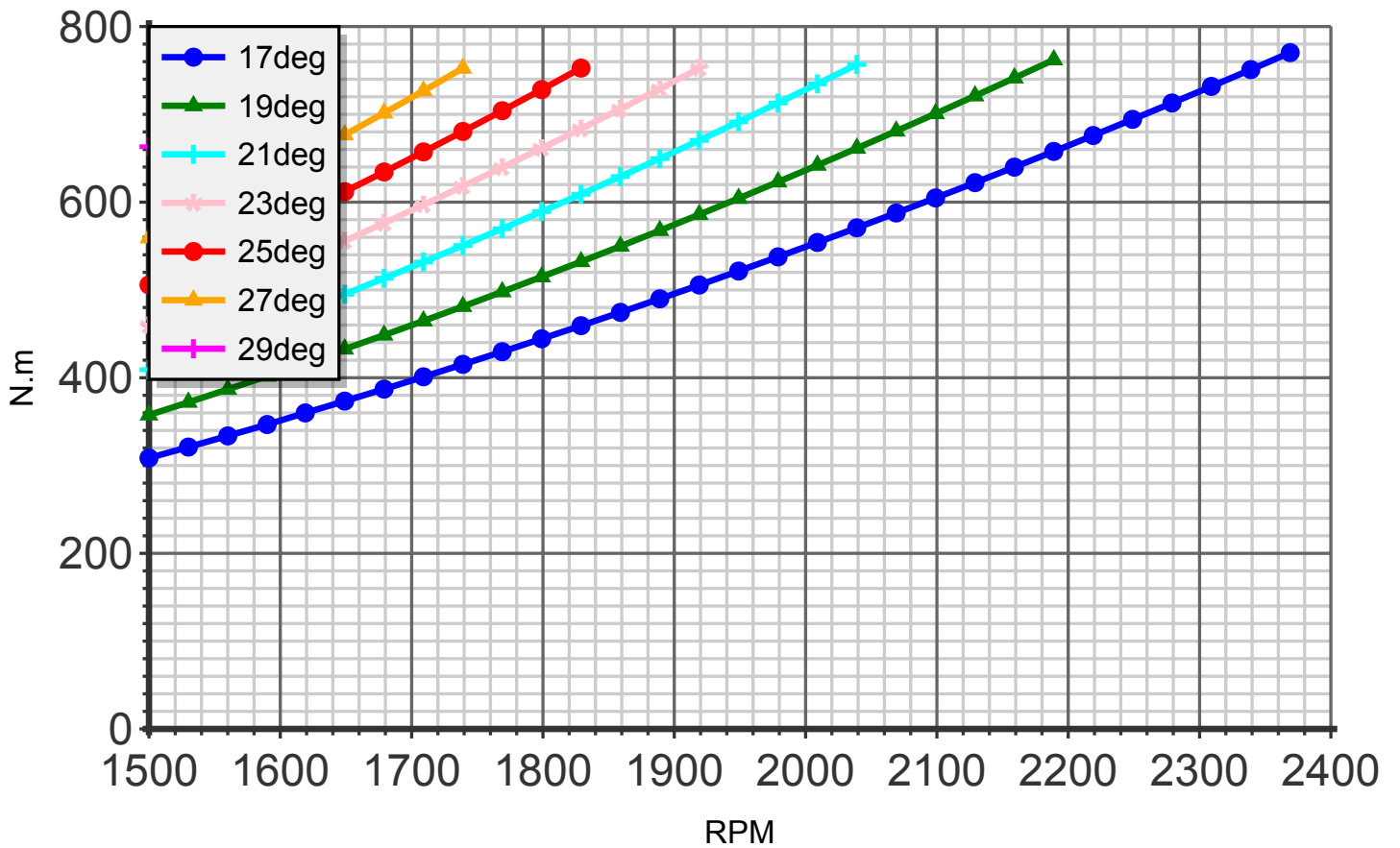
Torque (blade:5 diameter:209cm C4)
