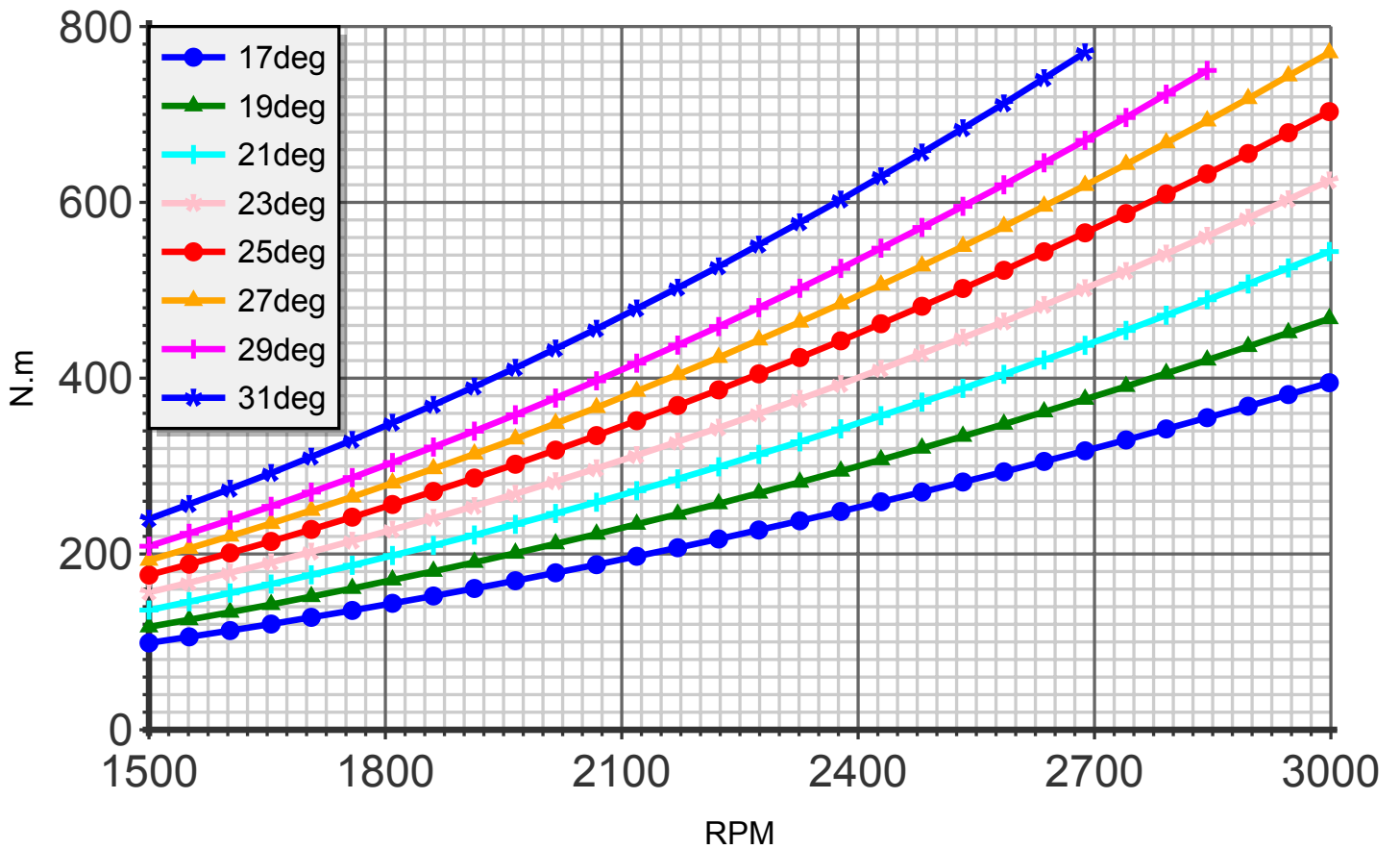
Torque (blade:5 diameter:164cm C4)
