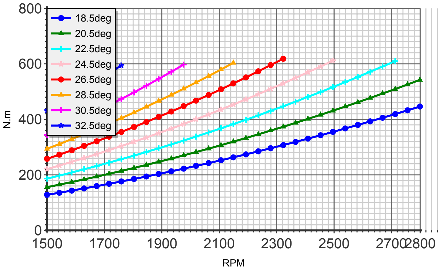
Torque (blade:4 diameter:177cm C8)
