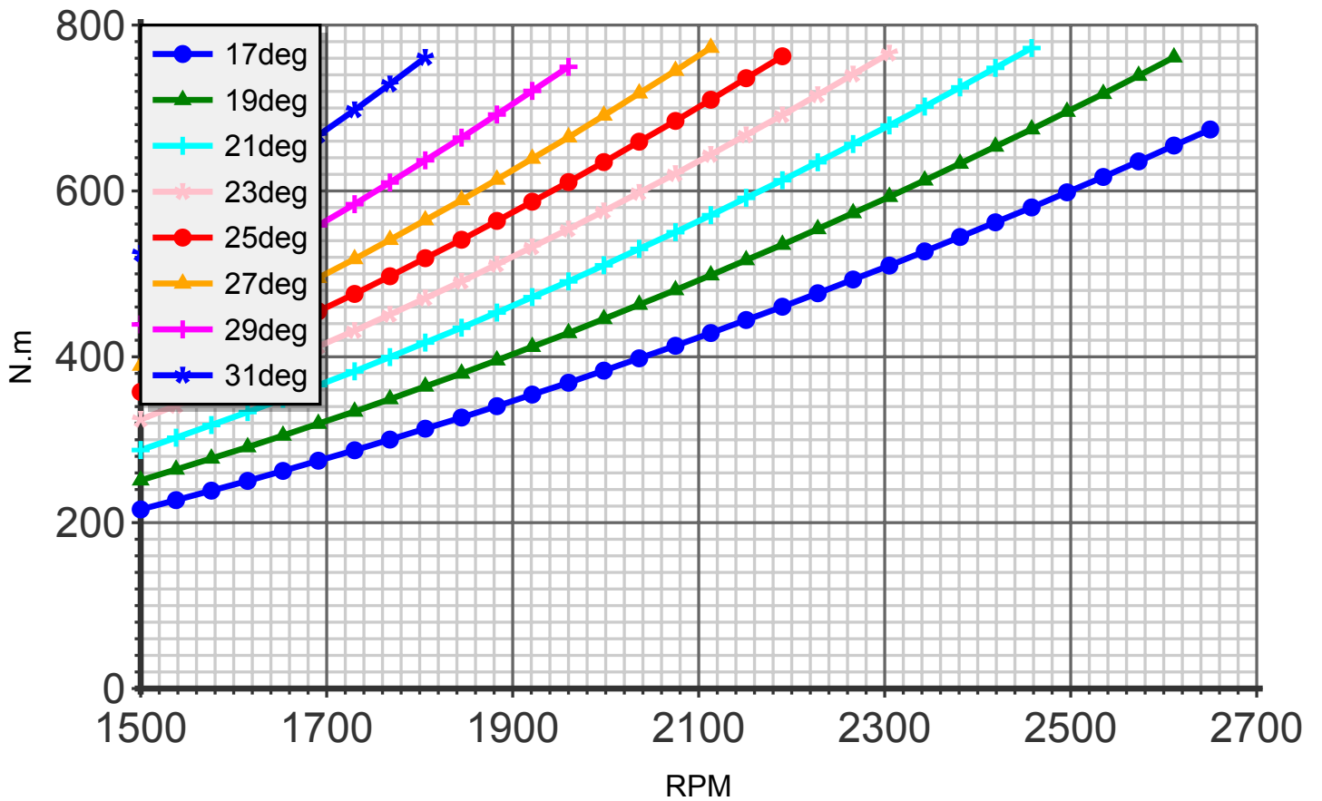
Torque (blade:5 diameter:189cm C4)
