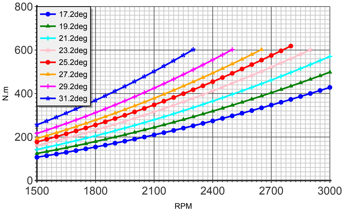
Torque (blade:4 diameter:167cm C4)
