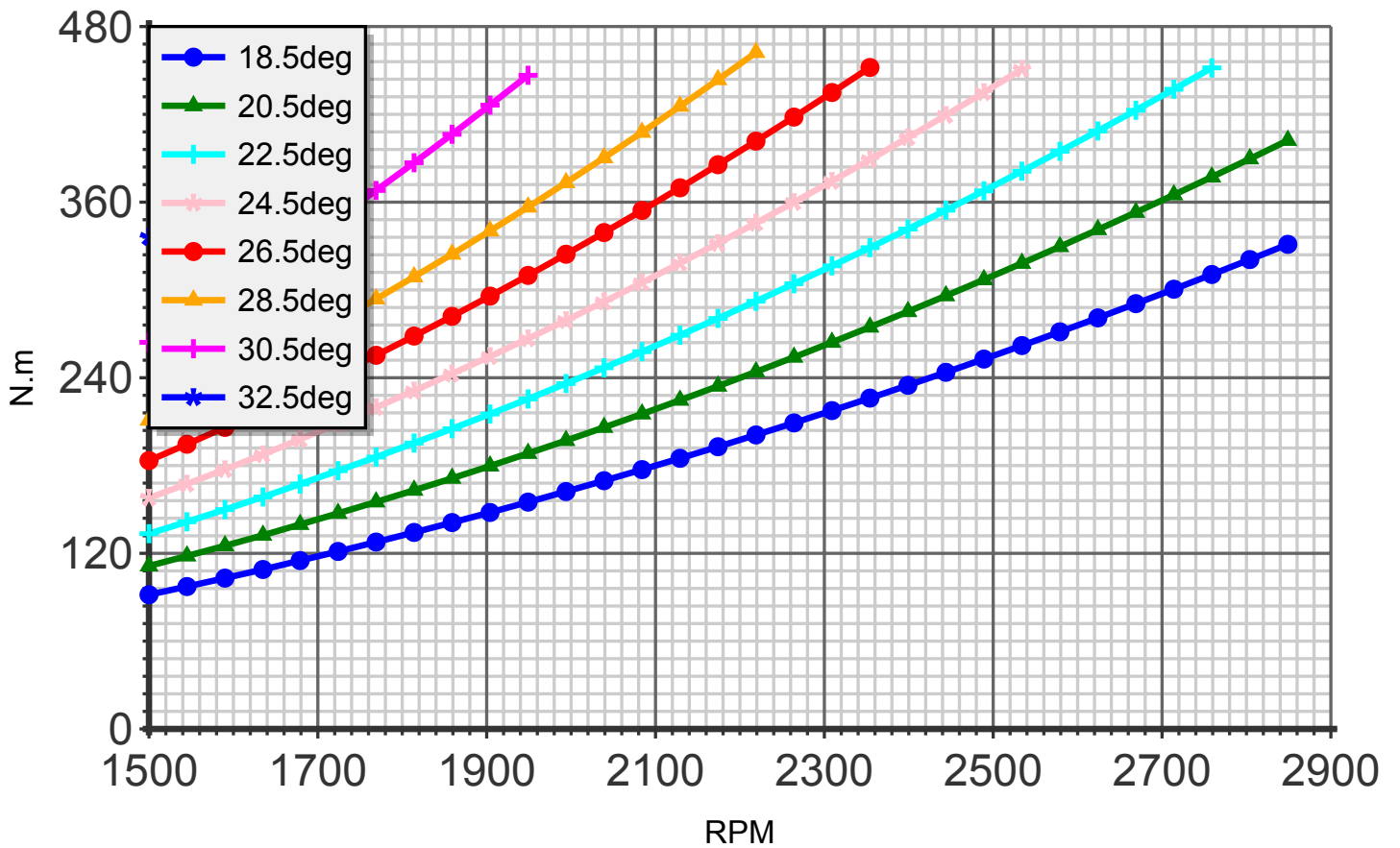
Torque (blade:3 diameter:175cm C8)
