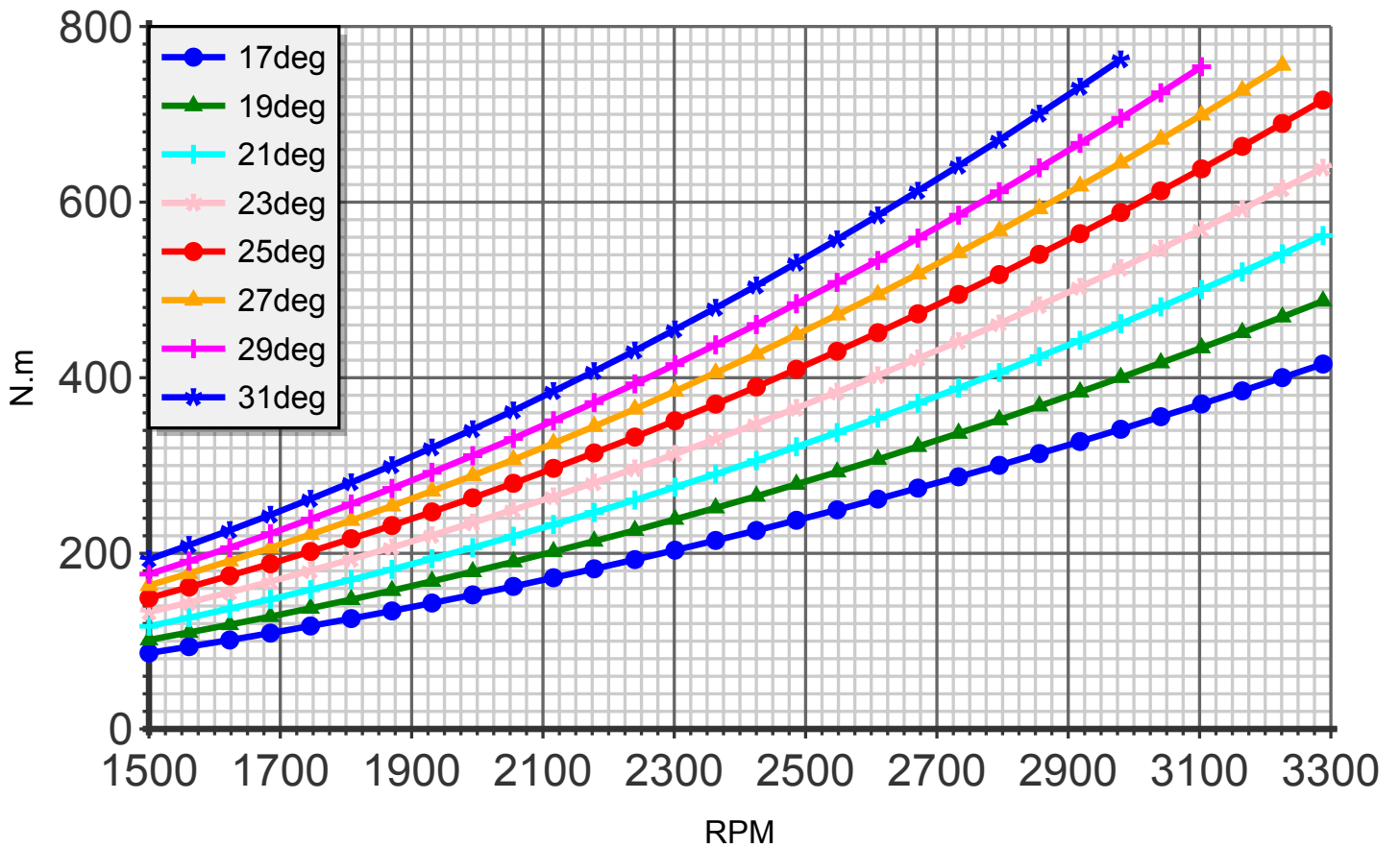
Torque (blade:5 diameter:149cm C4)
