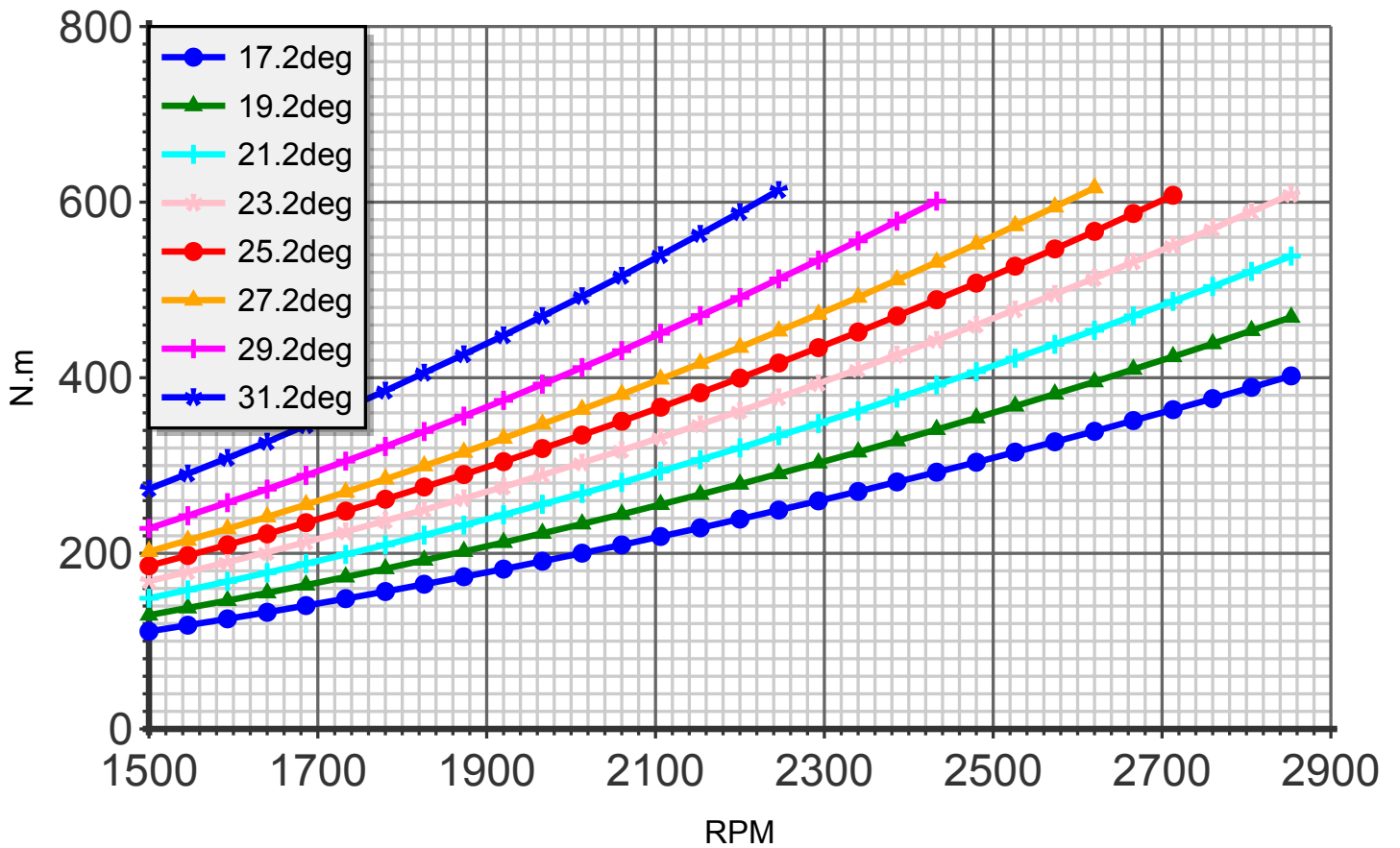
Torque (blade:4 diameter:172cm C4)
