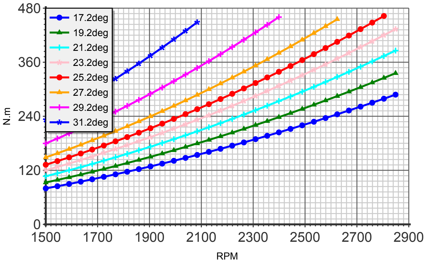
Torque (blade:3 diameter:175cm C4)
