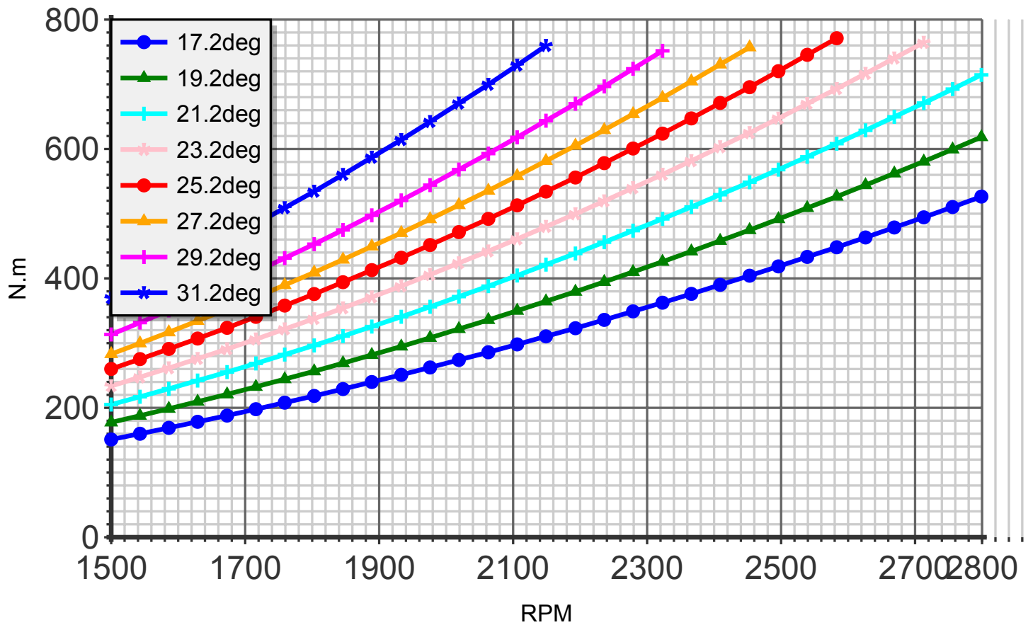
Torque (blade:5 diameter:179cm C4)
