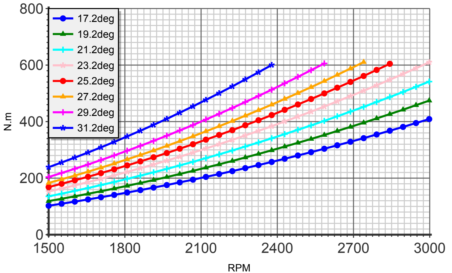
Torque (blade:4 diameter:162cm C4)
