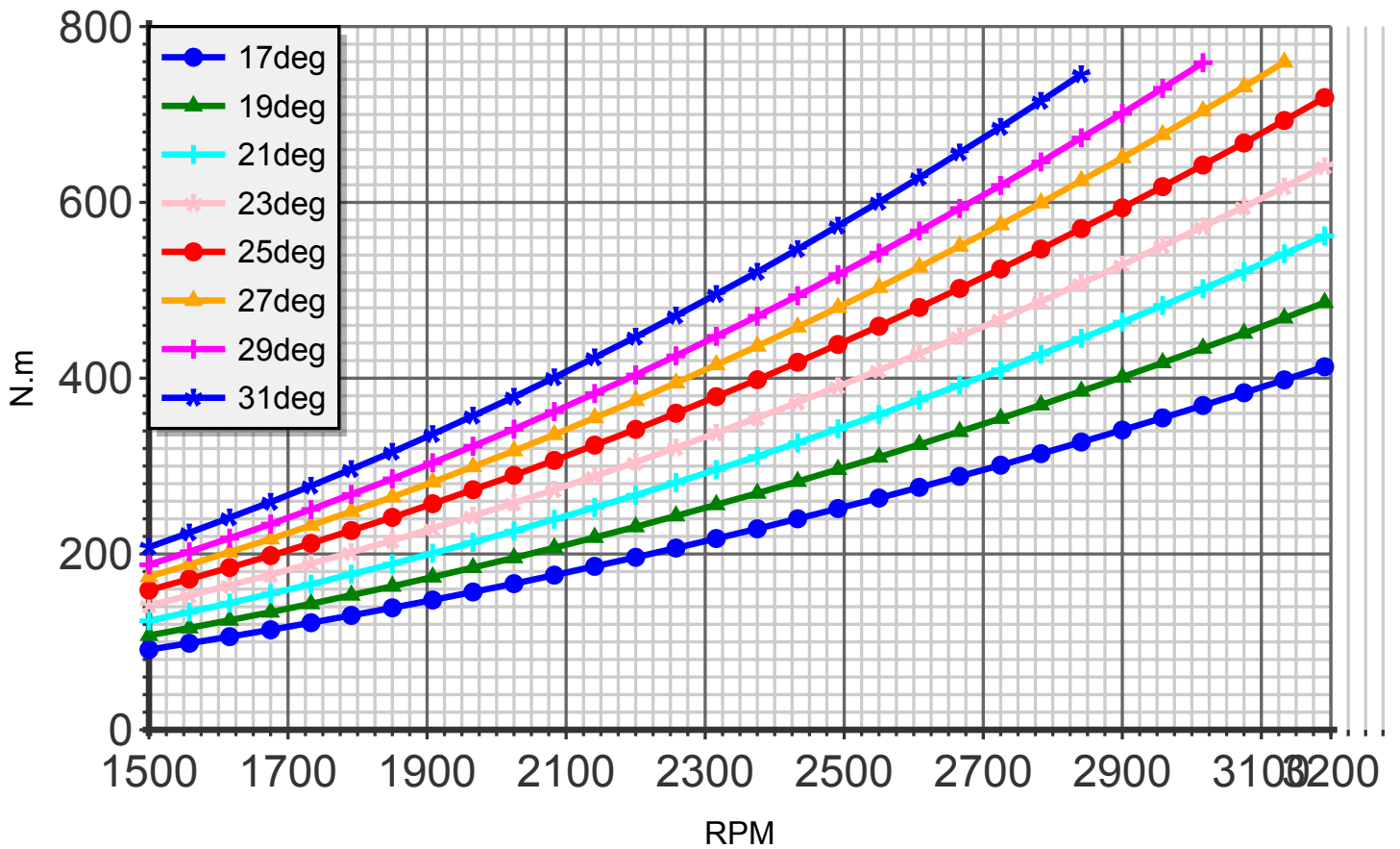
Torque (blade:5 diameter:154cm C4)
