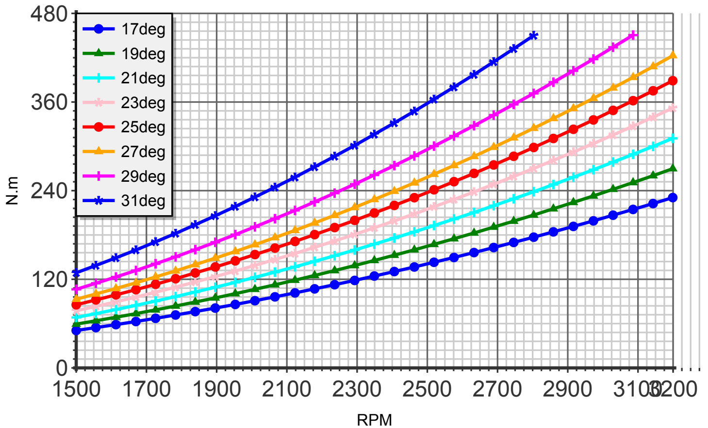
Torque (blade:3 diameter:155cm C4)
