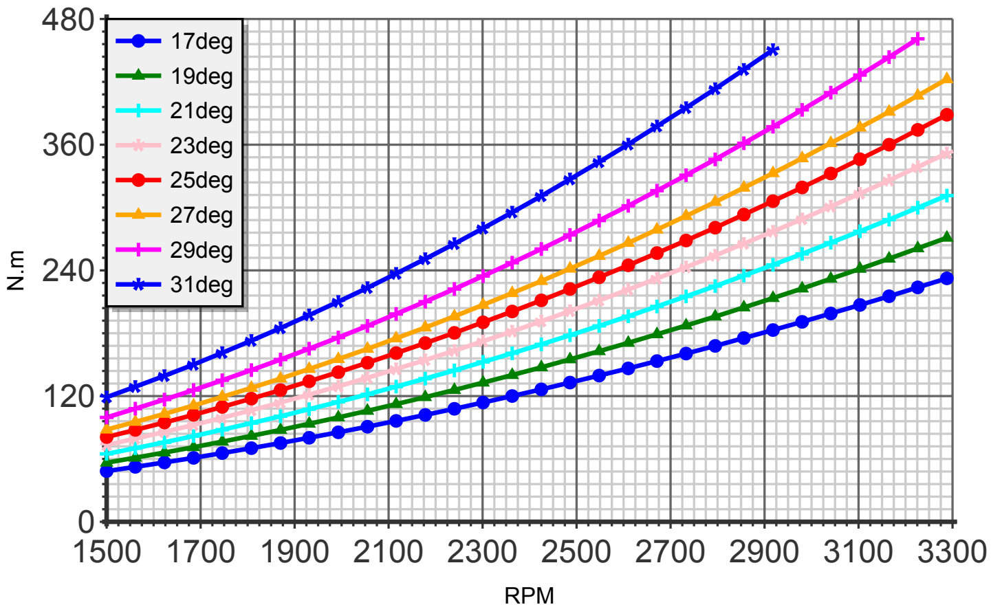
Torque (blade:3 diameter:150cm C4)
