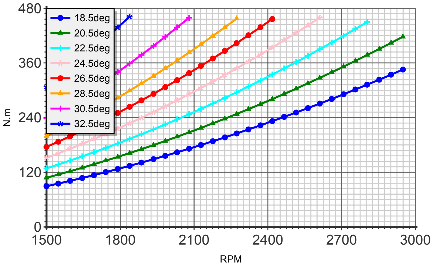
Torque (blade:3 diameter:170cm C8)
