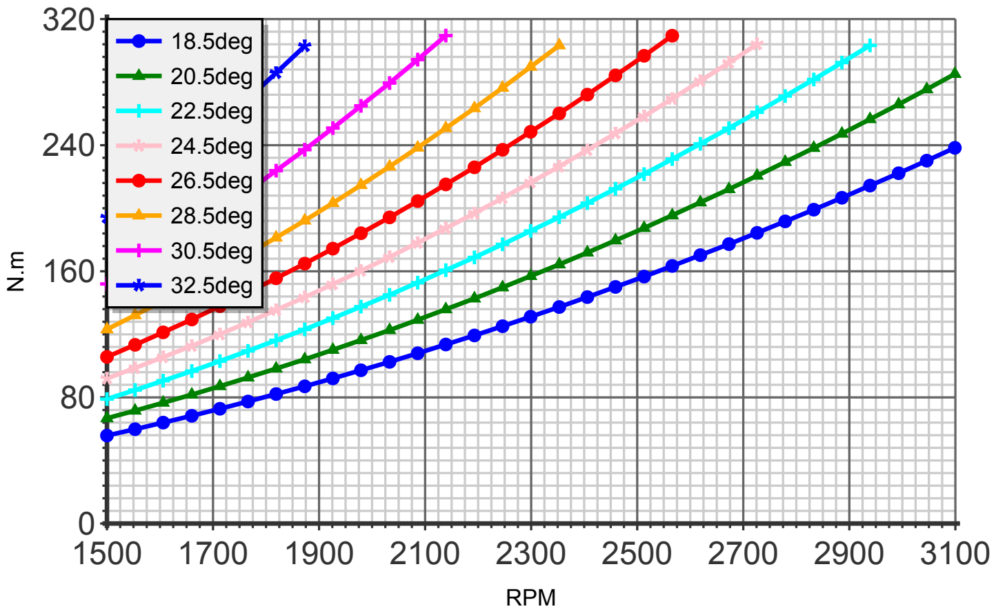
Torque (blade:2 diameter:160cm C8)
