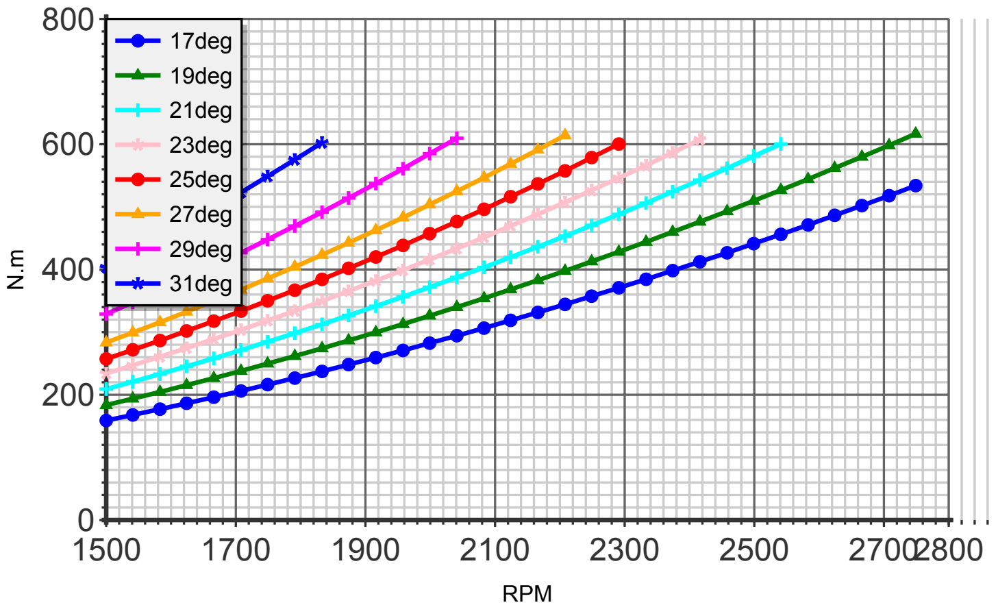
Torque (blade:4 diameter:182cm C4)
