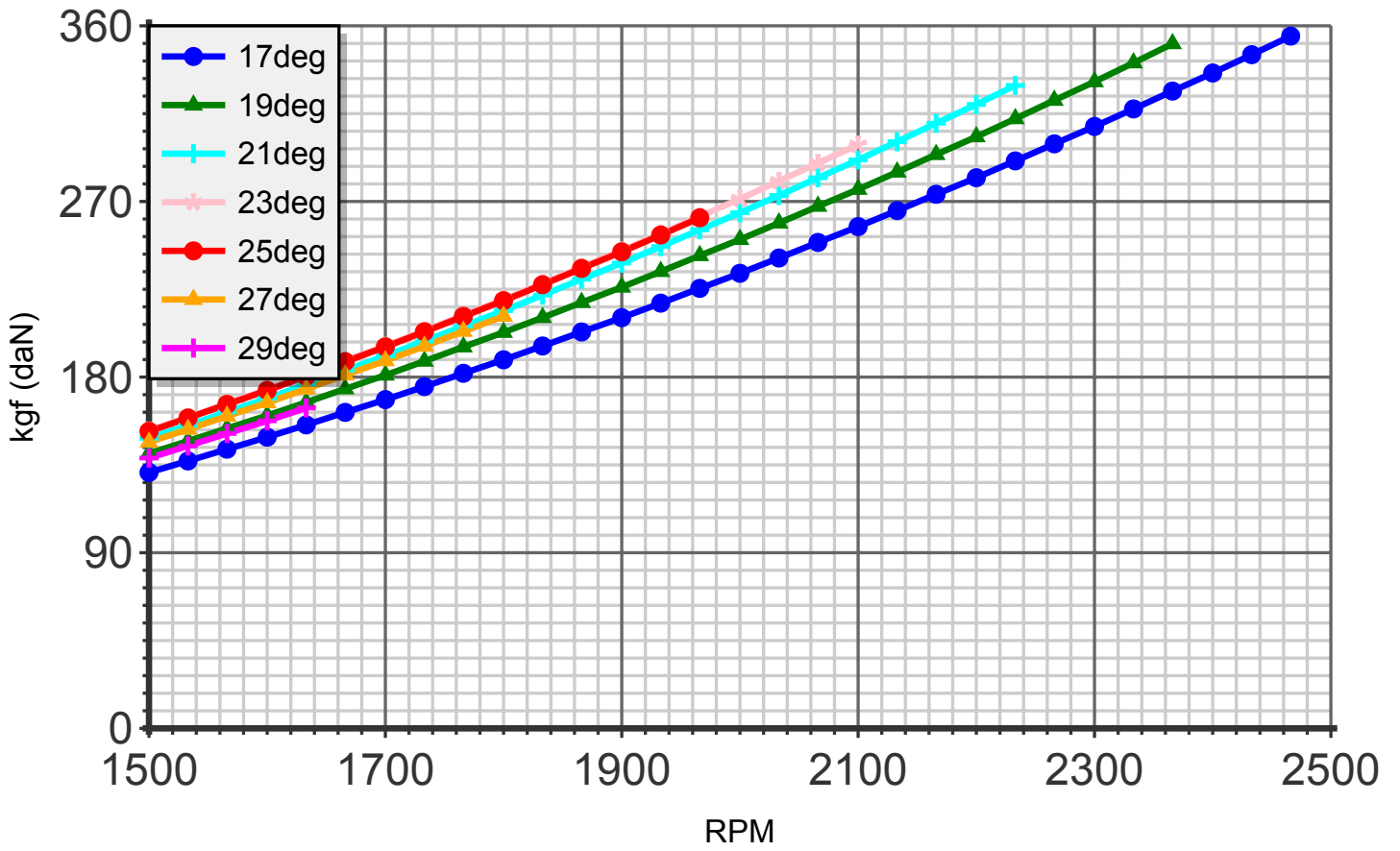
Thrust (blade:3 diameter:200cm C4)
