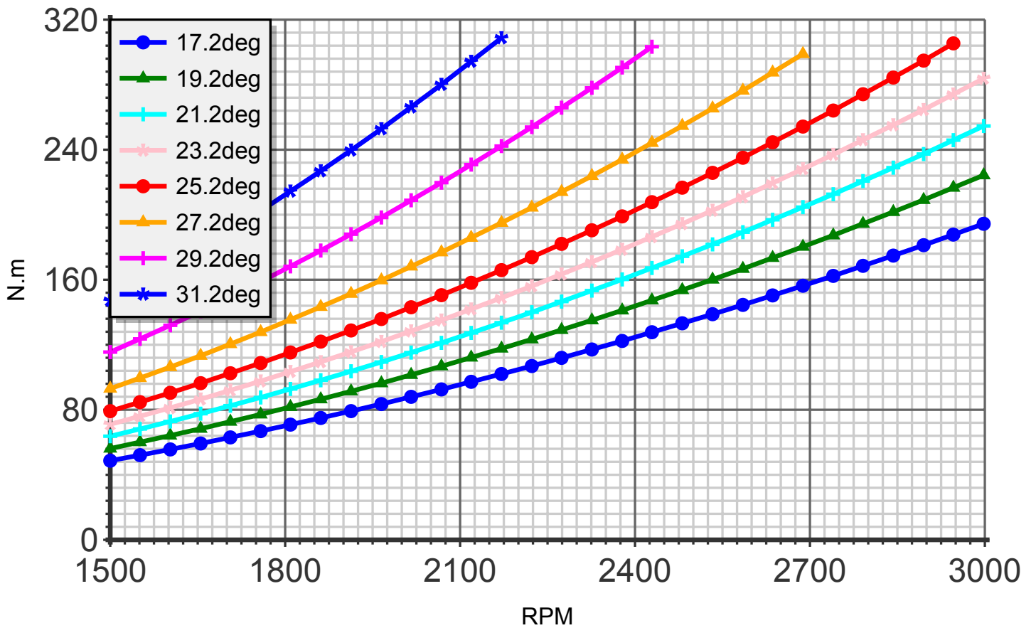
Torque (blade:2 diameter:165cm C4)
