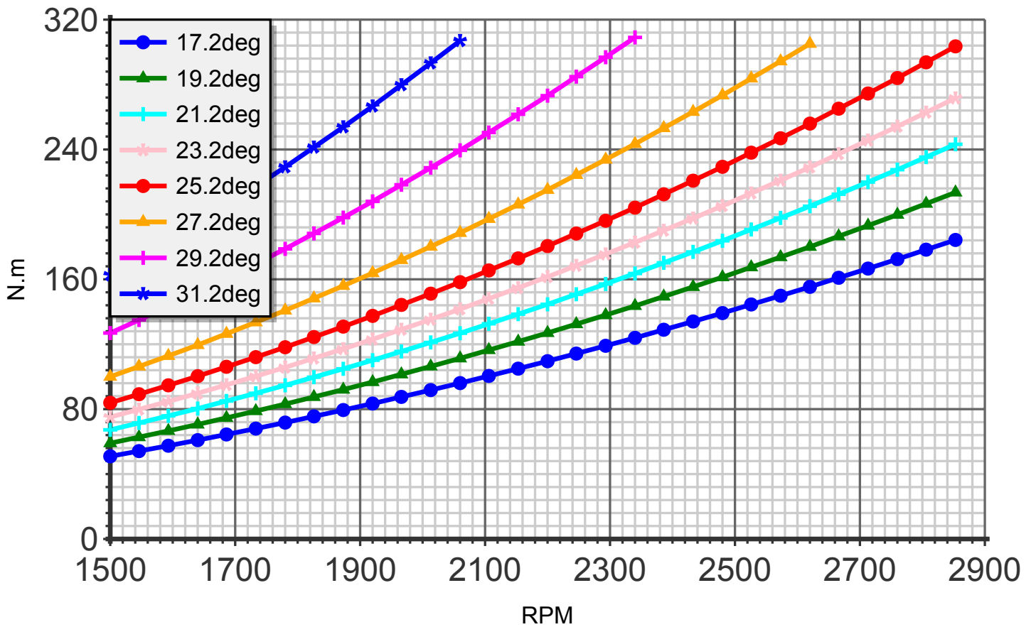
Torque (blade:2 diameter:172cm C4)
