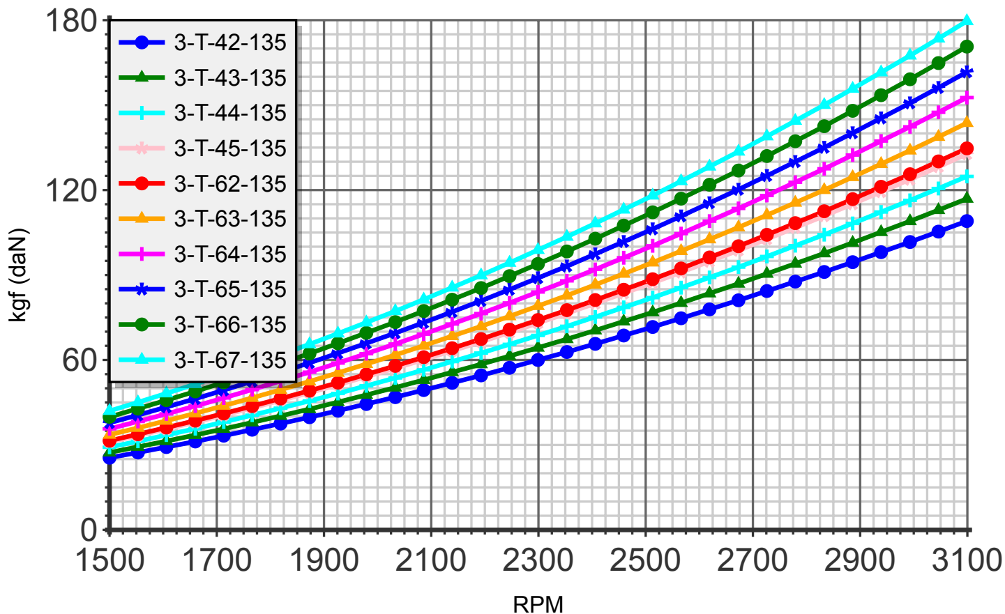
Thrust (blade:3 diameter:135cm)
