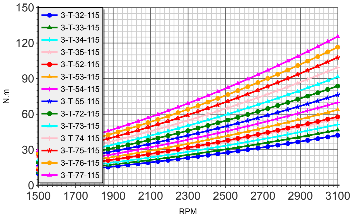
Torque (blade:3 diameter:115cm)
