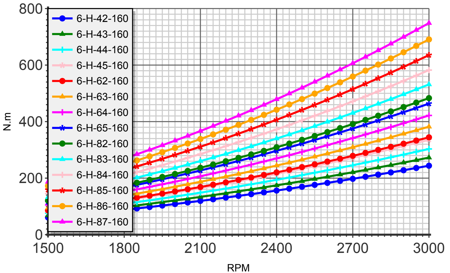
Torque (blade:6 diameter:160cm)
