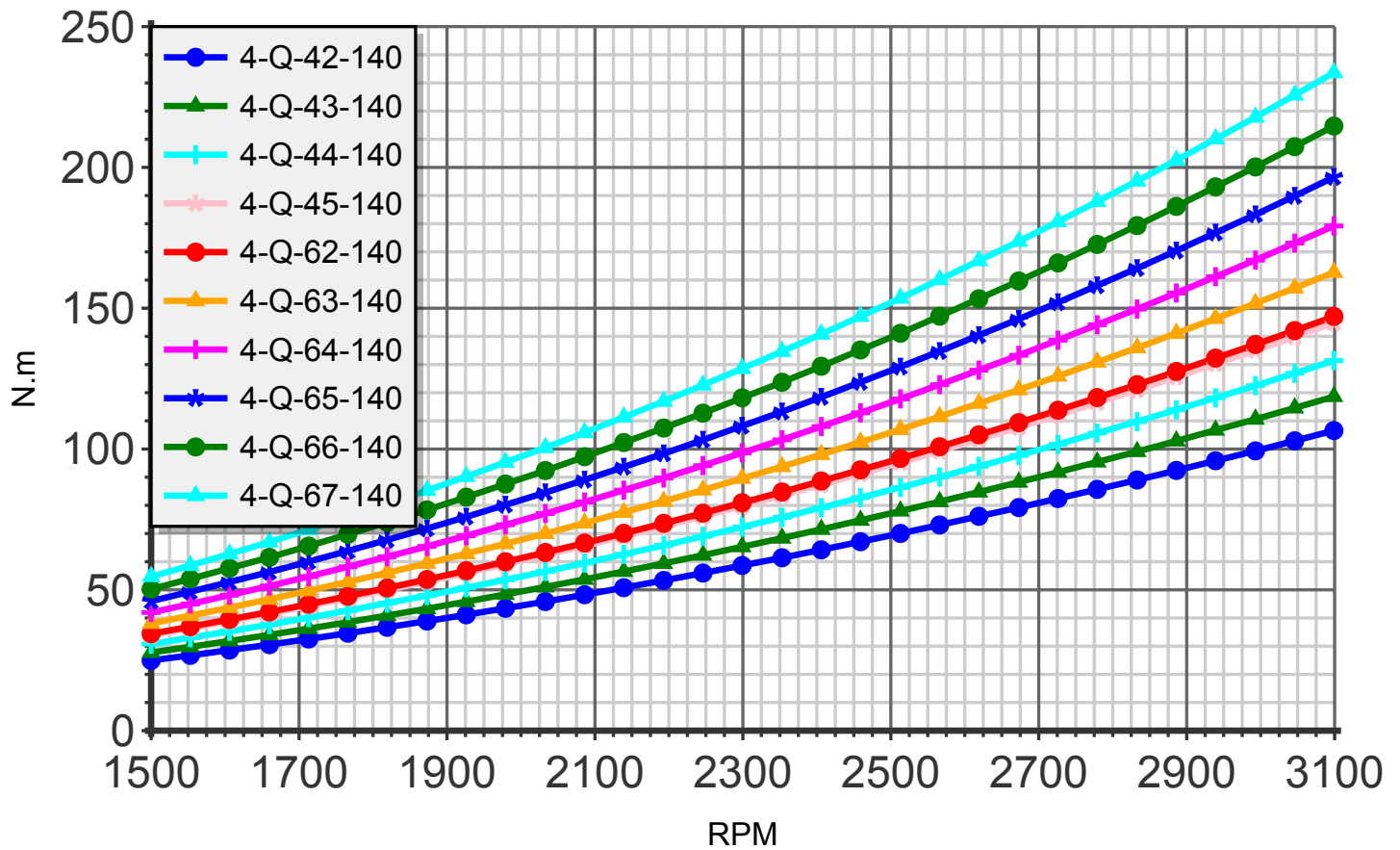
Torque (blade:4 diameter:140cm)
