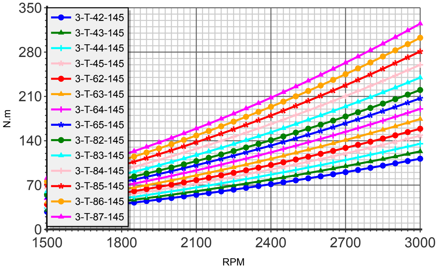
Torque (blade:3 diameter:145cm)
