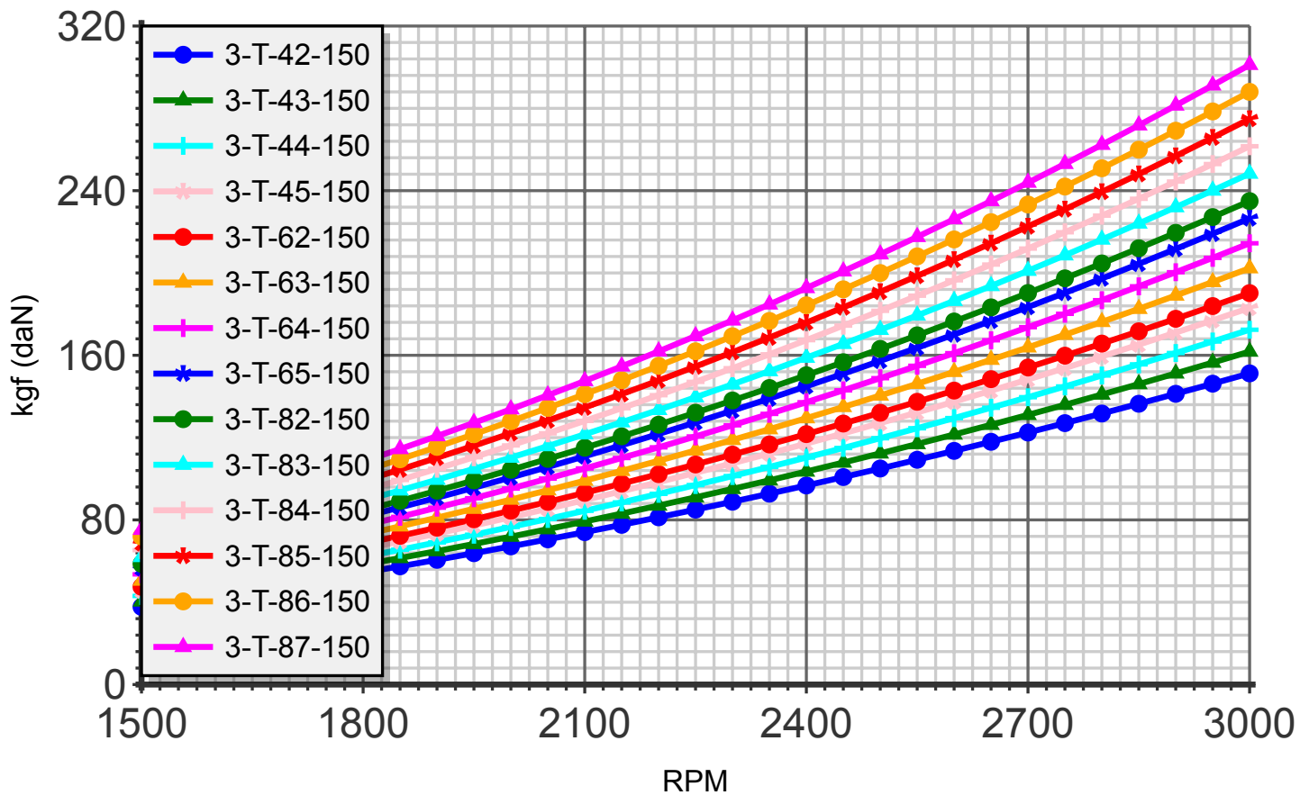
Thrust (blade:3 diameter:150cm)
