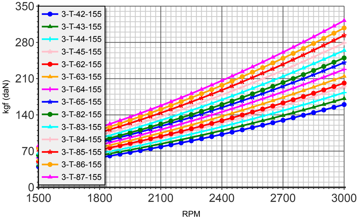
Thrust (blade:3 diameter:155cm)
