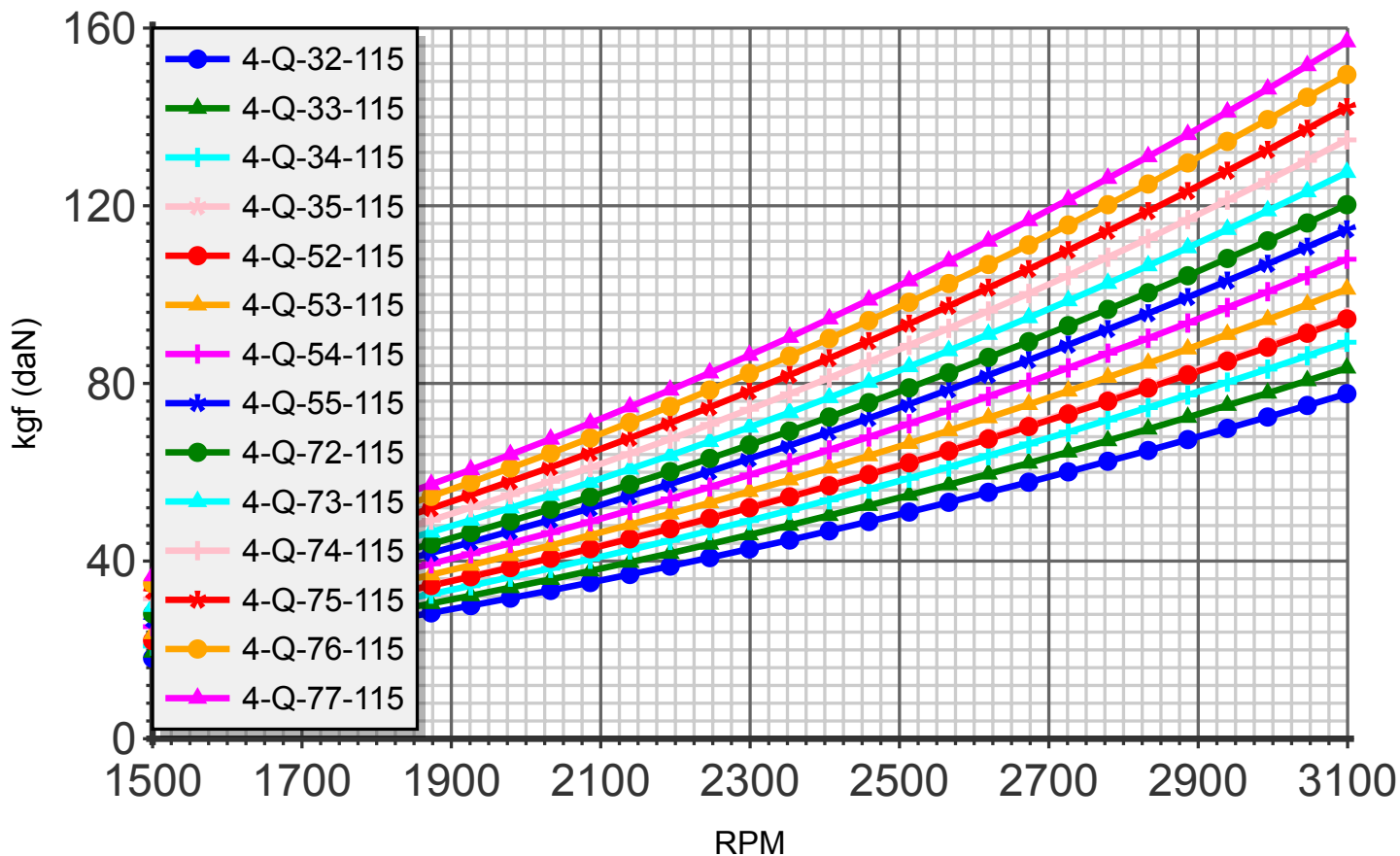
Thrust (blade:4 diameter:115cm)
