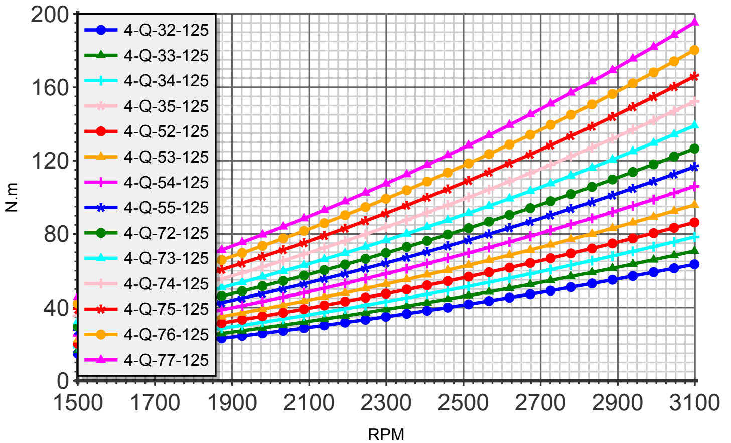
Torque (blade:4 diameter:125cm)
