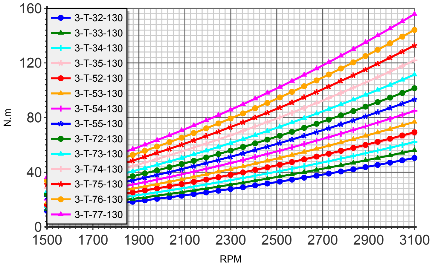
Torque (blade:3 diameter:130cm)
