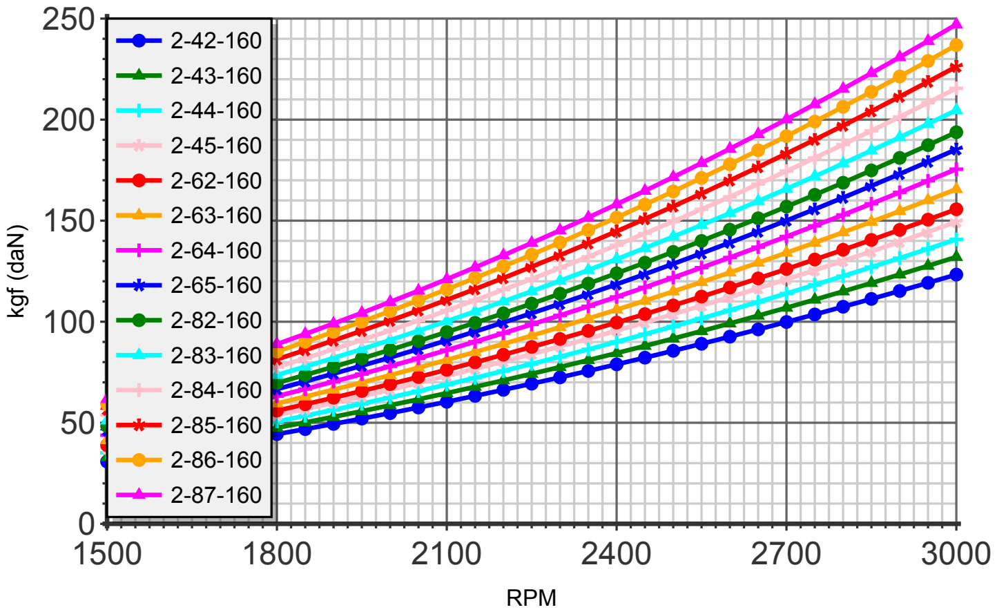
Thrust (blade:2 diameter:160cm)
