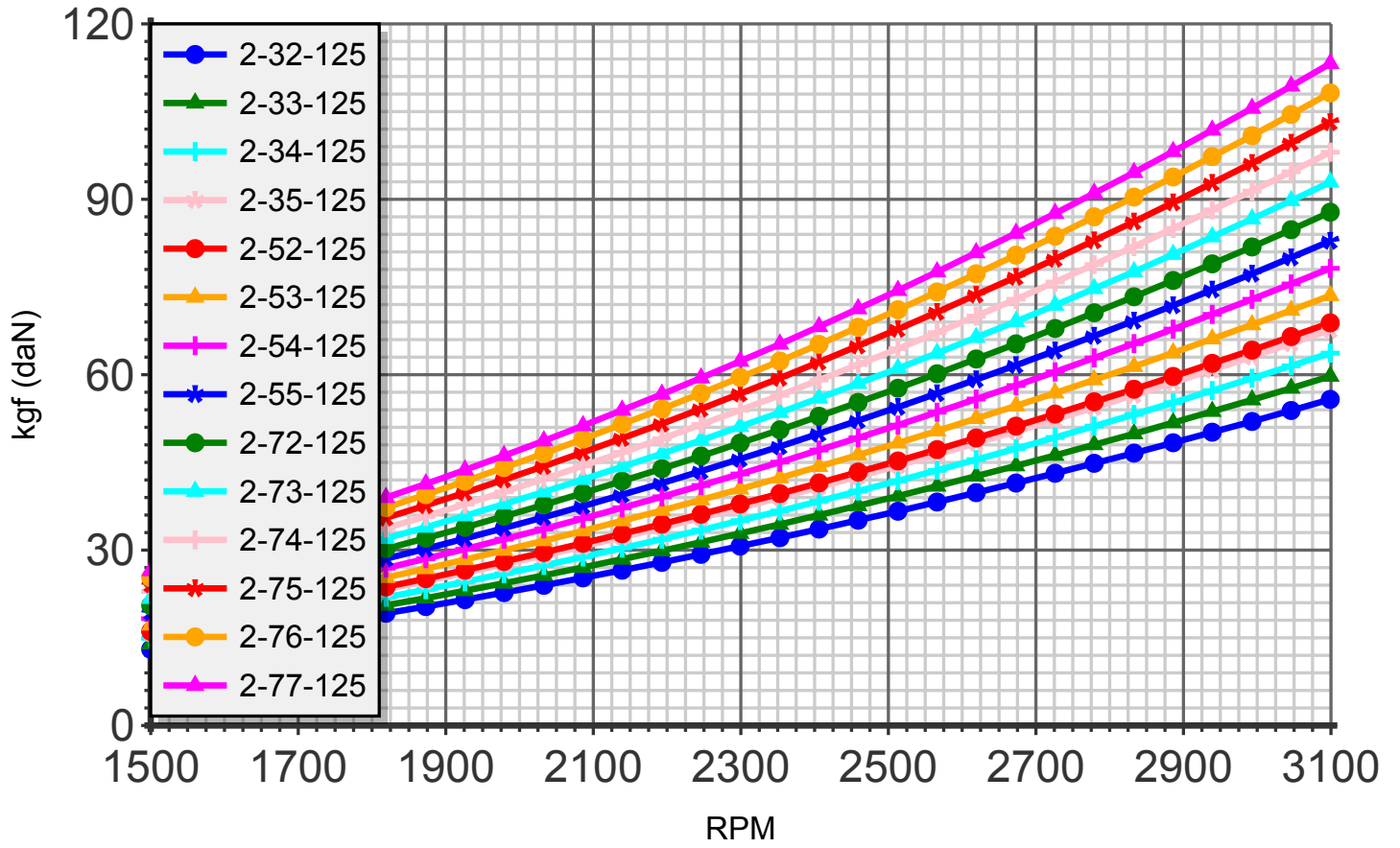
Thrust (blade:2 diameter:125cm)
