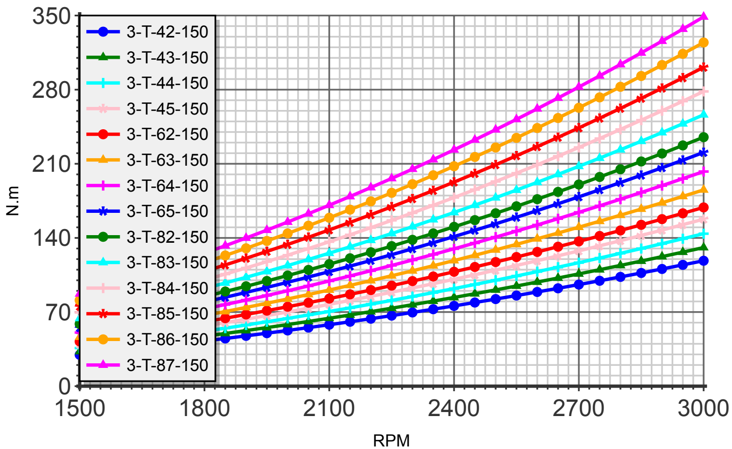
Torque (blade:3 diameter:150cm)
