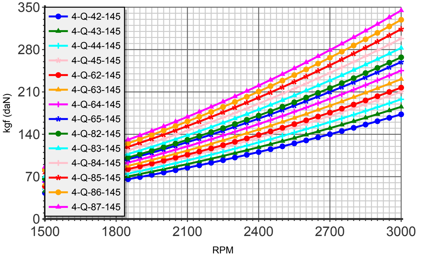
Thrust (blade:4 diameter:145cm)
