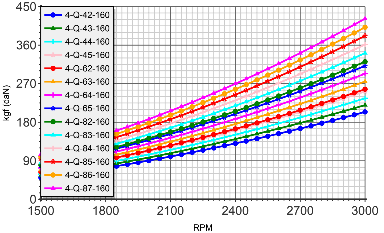
Thrust (blade:4 diameter:160cm)
