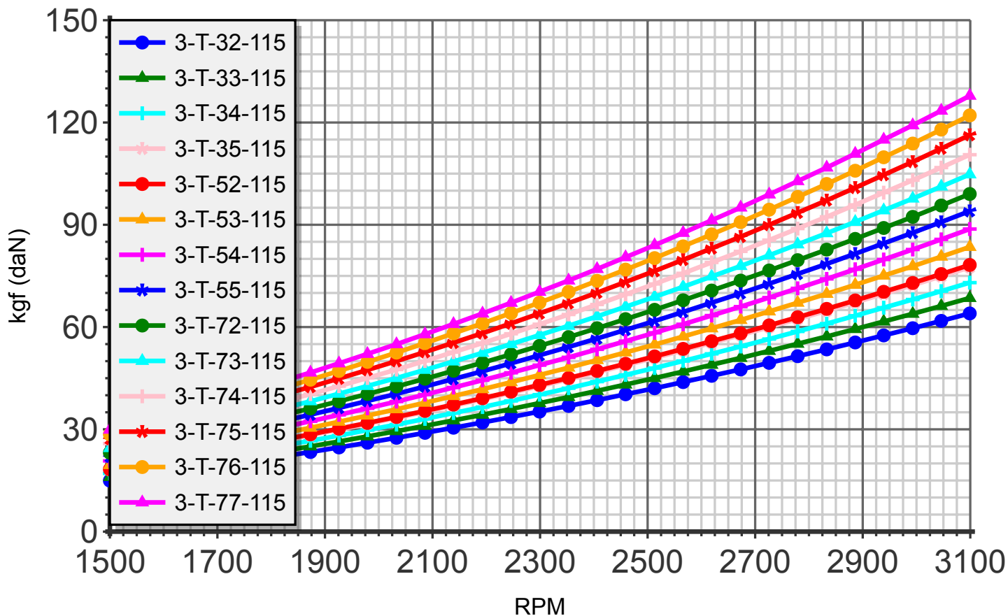
Thrust (blade:3 diameter:115cm)
