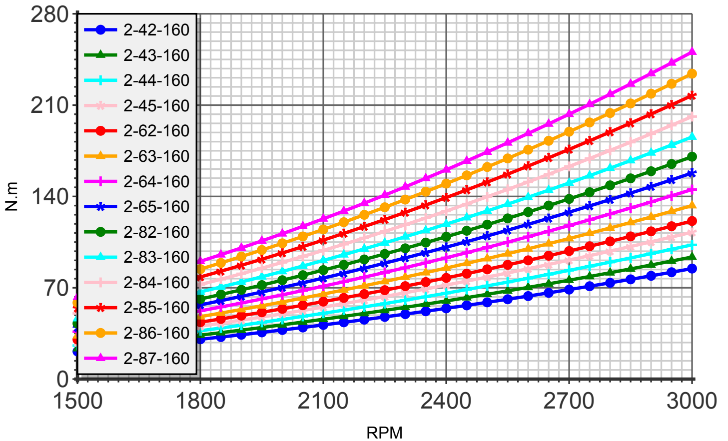
Torque (blade:2 diameter:160cm)
