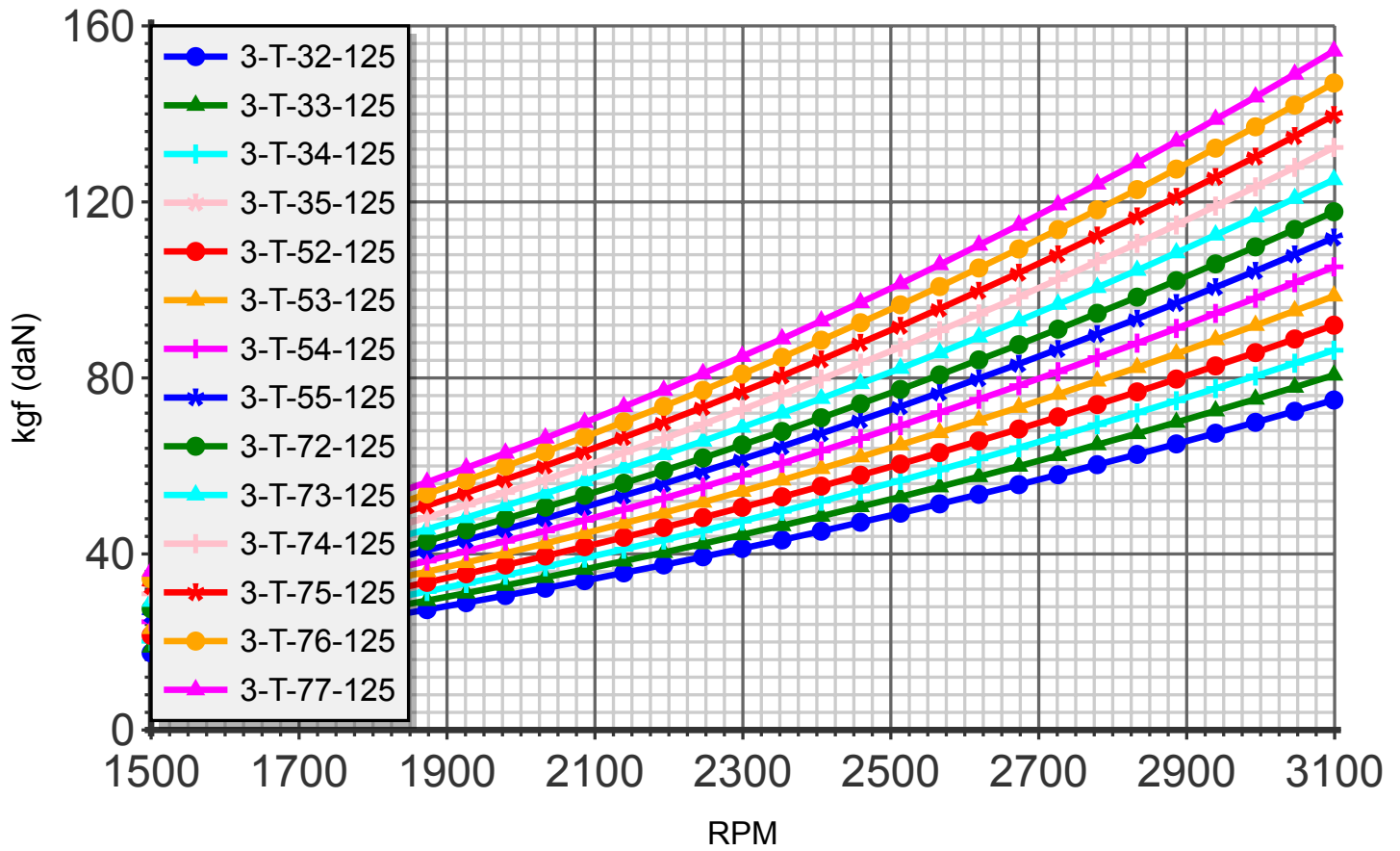
Thrust (blade:3 diameter:125cm)
