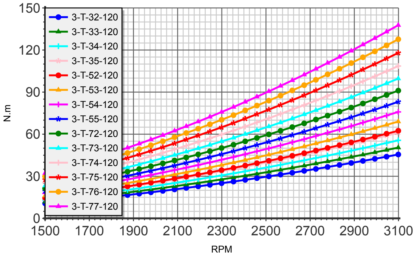
Torque (blade:3 diameter:120cm)
