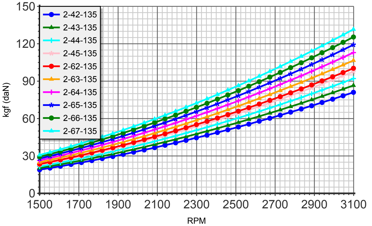
Thrust (blade:2 diameter:135cm)
