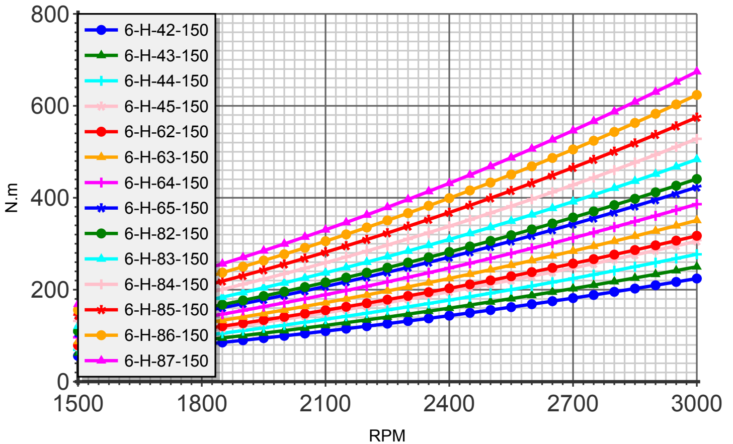
Torque (blade:6 diameter:150cm)
