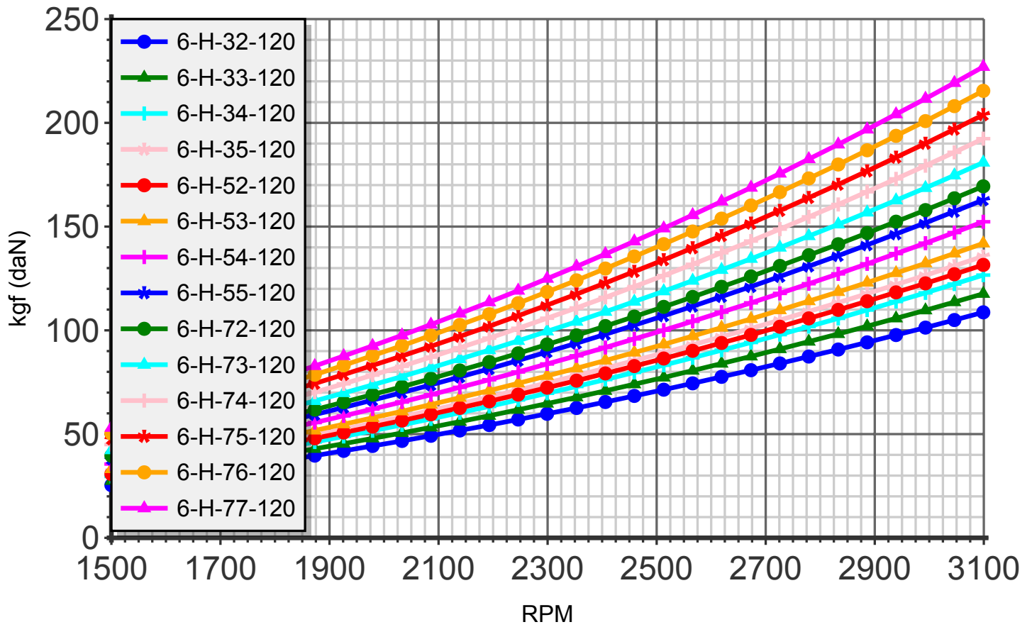
Thrust (blade:6 diameter:120cm)
