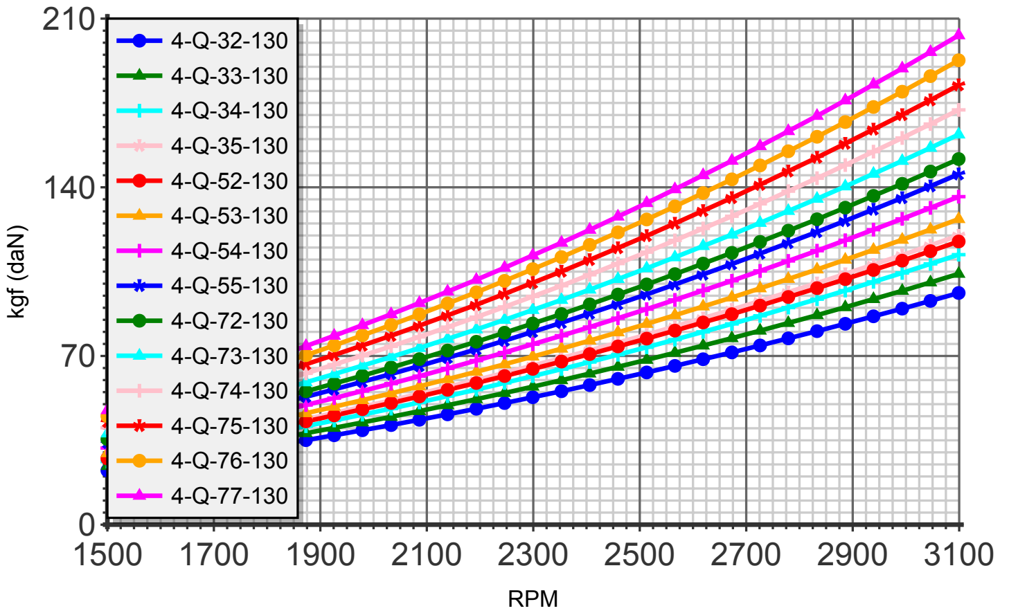
Thrust (blade:4 diameter:130cm)
