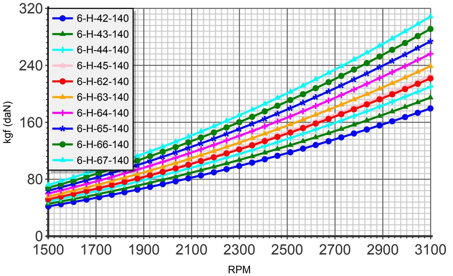
Thrust (blade:6 diameter:140cm)
