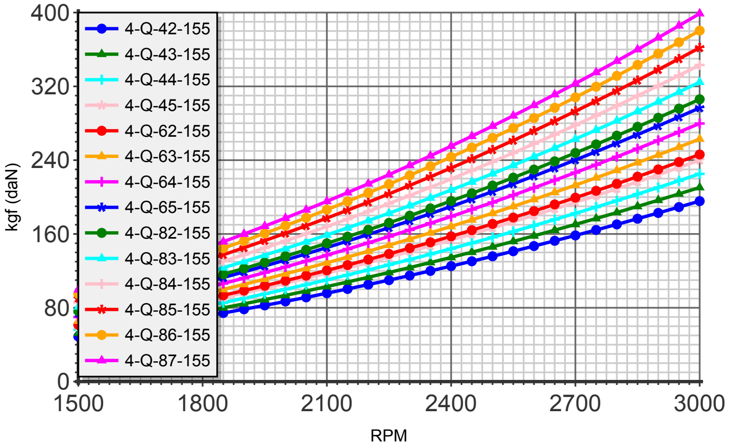
Thrust (blade:4 diameter:155cm)
