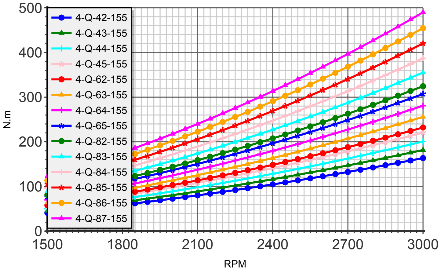
Torque (blade:4 diameter:155cm)
