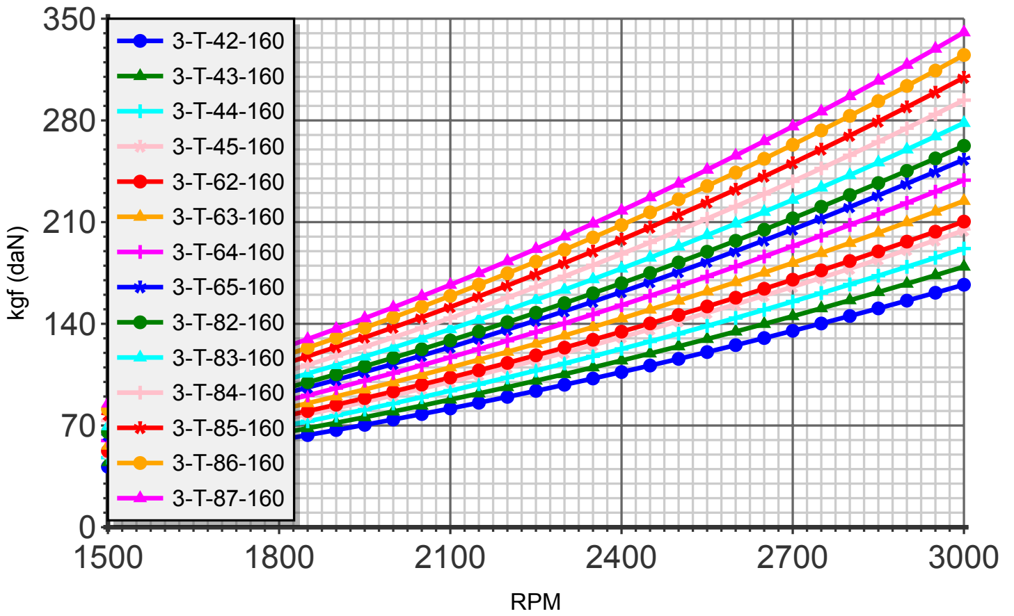
Thrust (blade:3 diameter:160cm)
