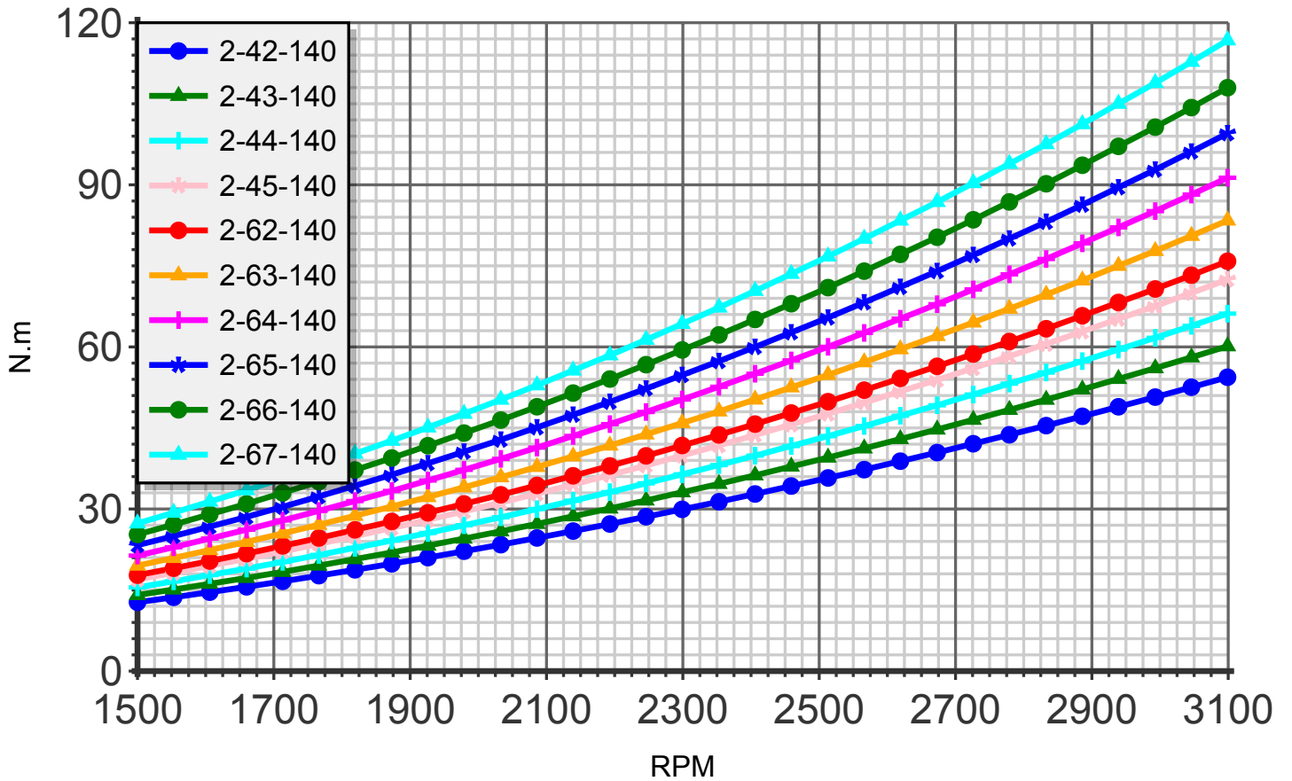
Torque (blade:2 diameter:140cm)
