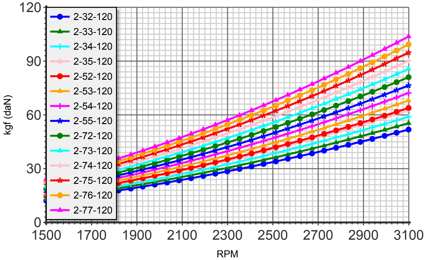
Thrust (blade:2 diameter:120cm)
