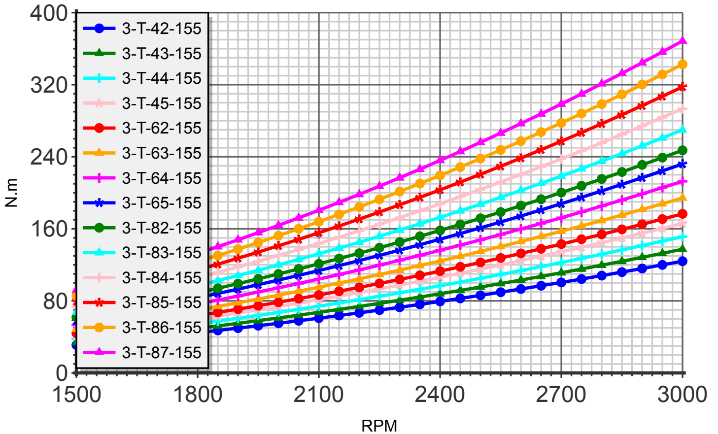
Torque (blade:3 diameter:155cm)
