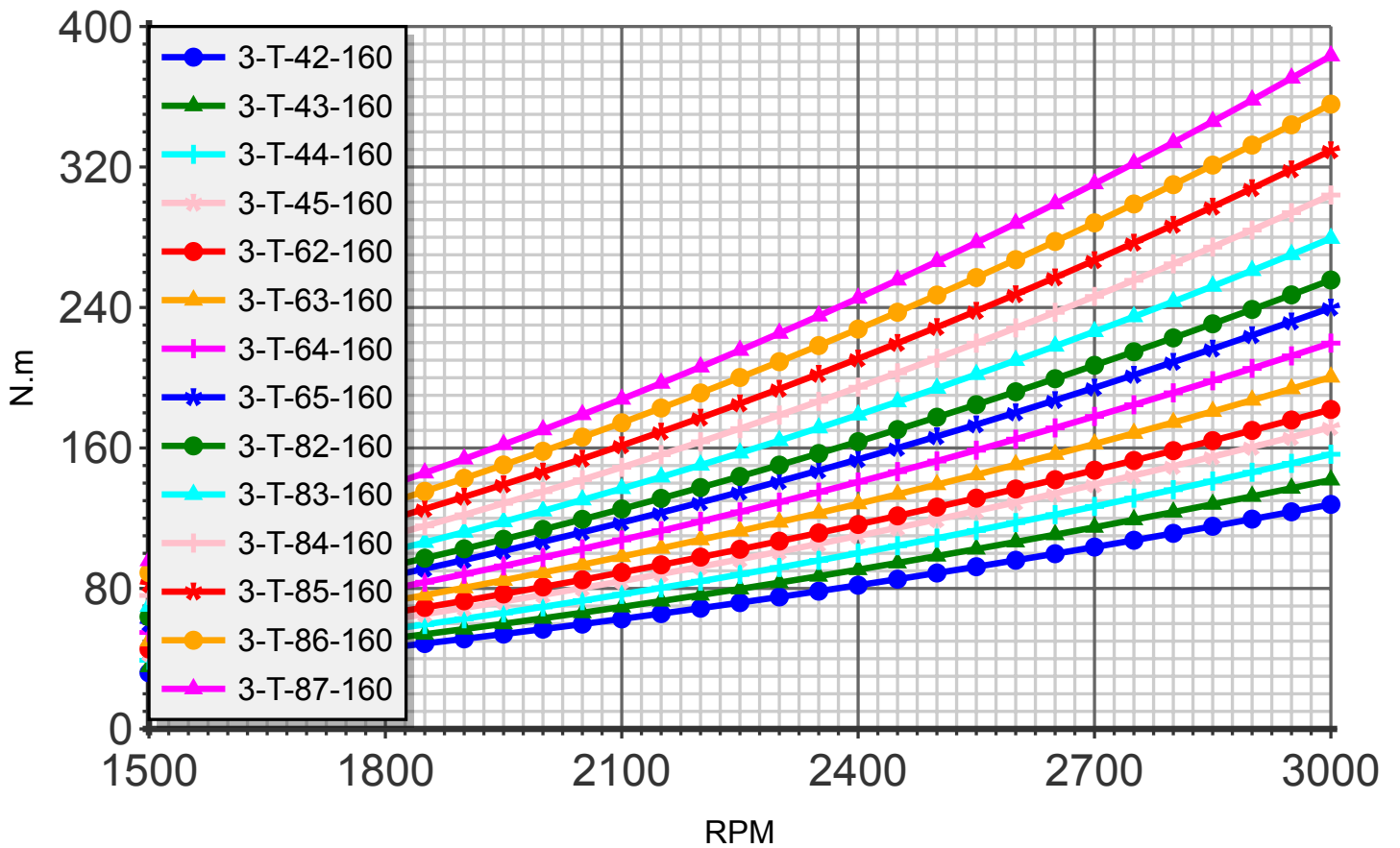
Torque (blade:3 diameter:160cm)
