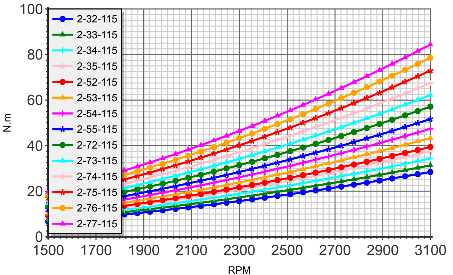
Torque (blade:2 diameter:115cm)
