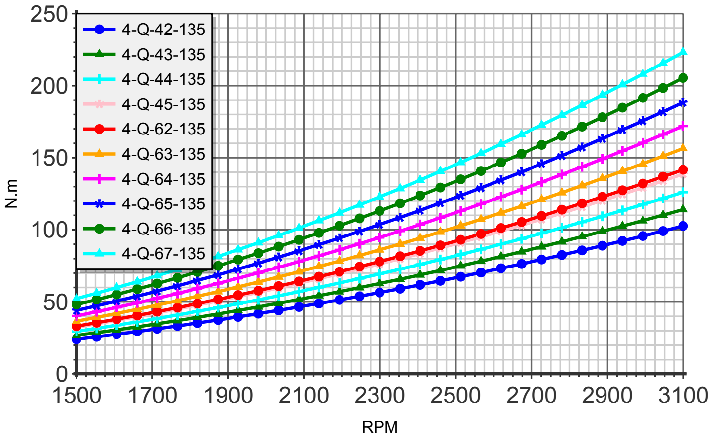
Torque (blade:4 diameter:135cm)
