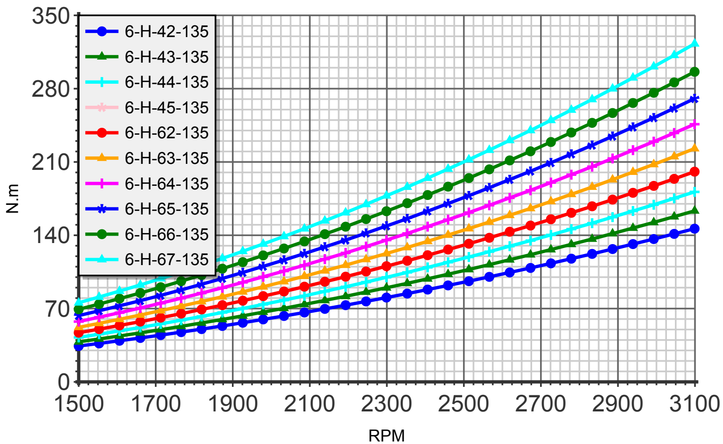
Torque (blade:6 diameter:135cm)
