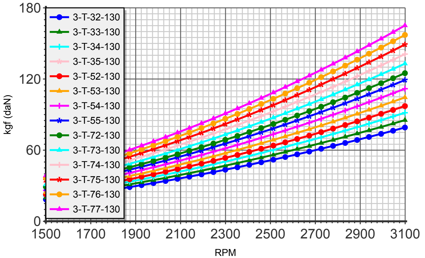
Thrust (blade:3 diameter:130cm)
